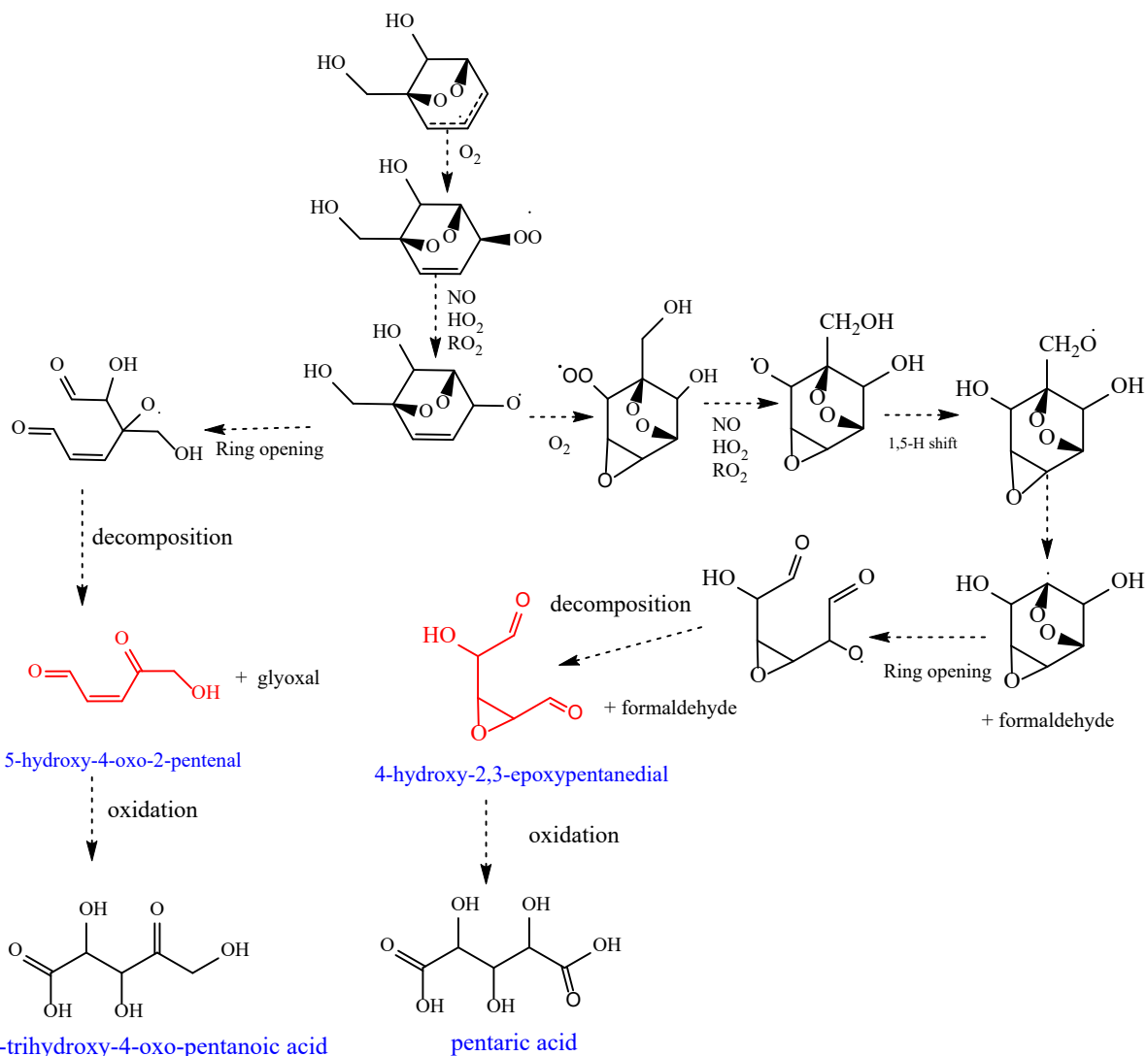
2,3,5-trihydroxy-4-oxo-pentanoic acid
