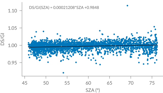
(c) Andøya seasonal effect on GI
