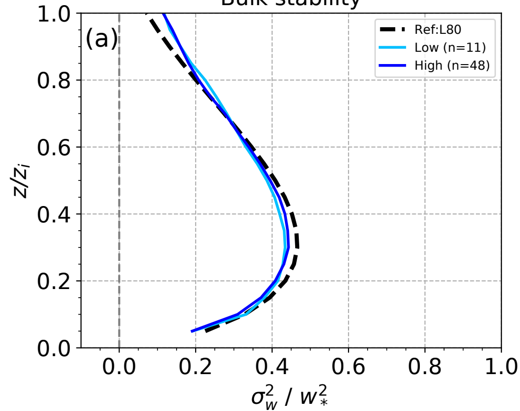
Bulk stability
