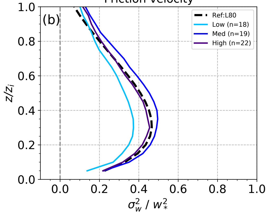
Friction velocity
