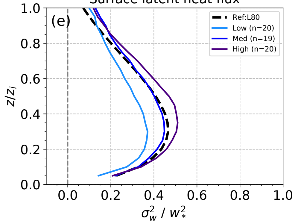
Surface latent heat flux
