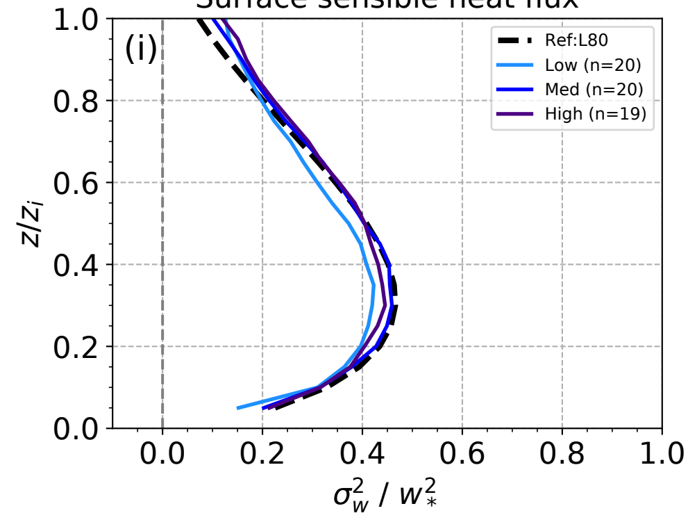
Surface sensible heat flux
