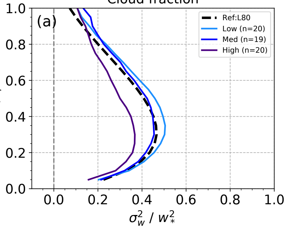
Cloud fraction
