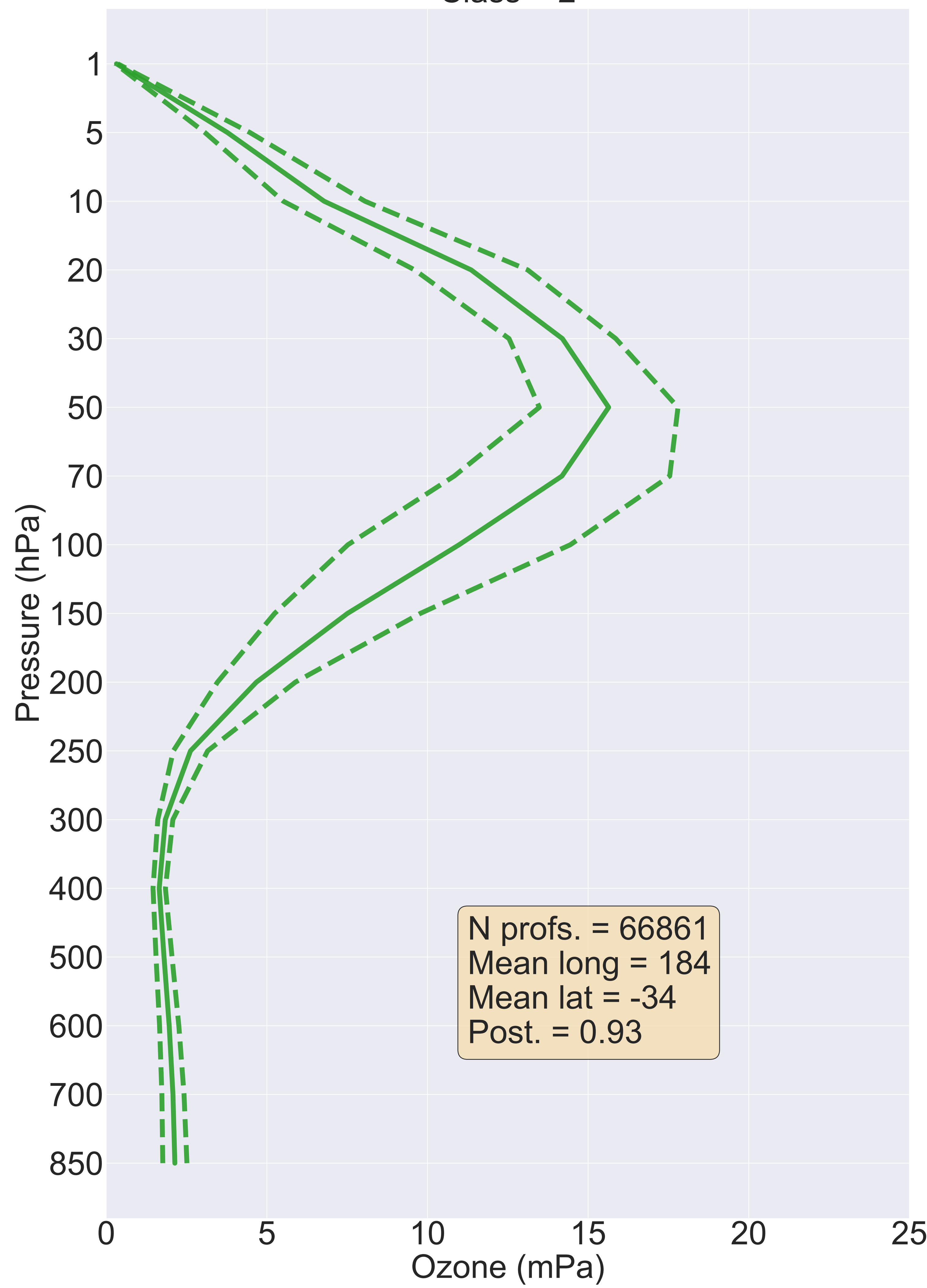
Class = 2
