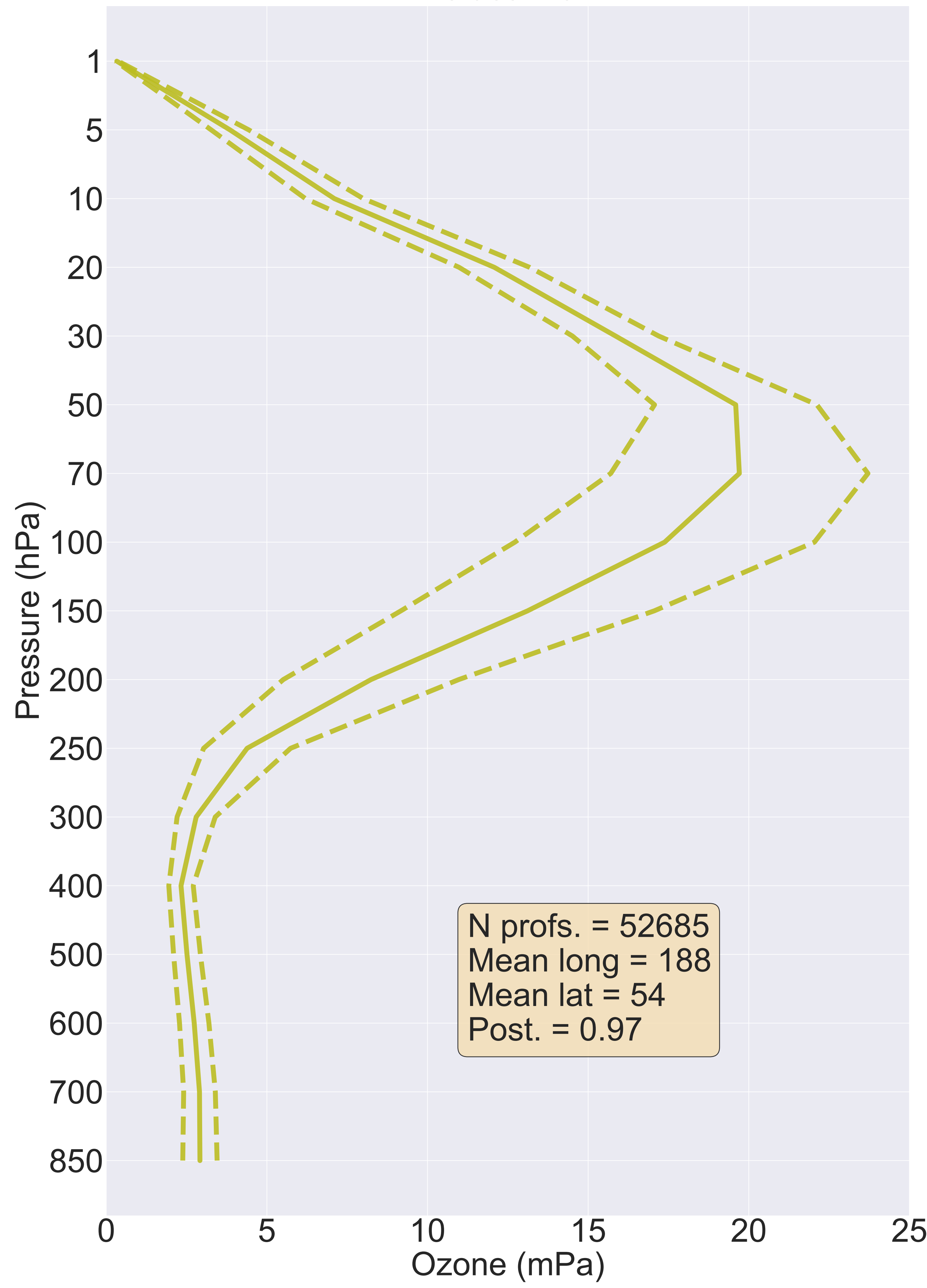
Class = 5
