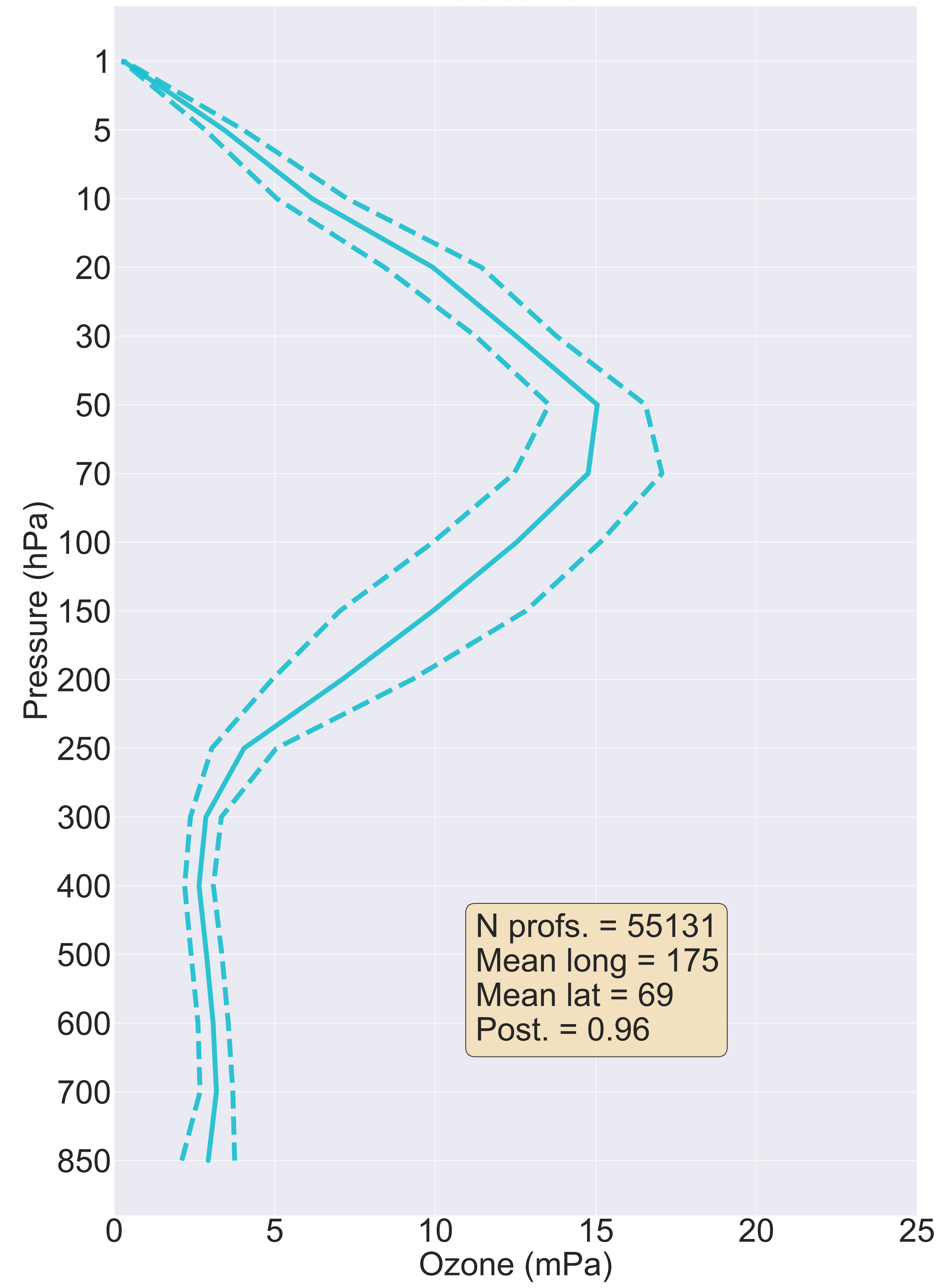
Class = 6
