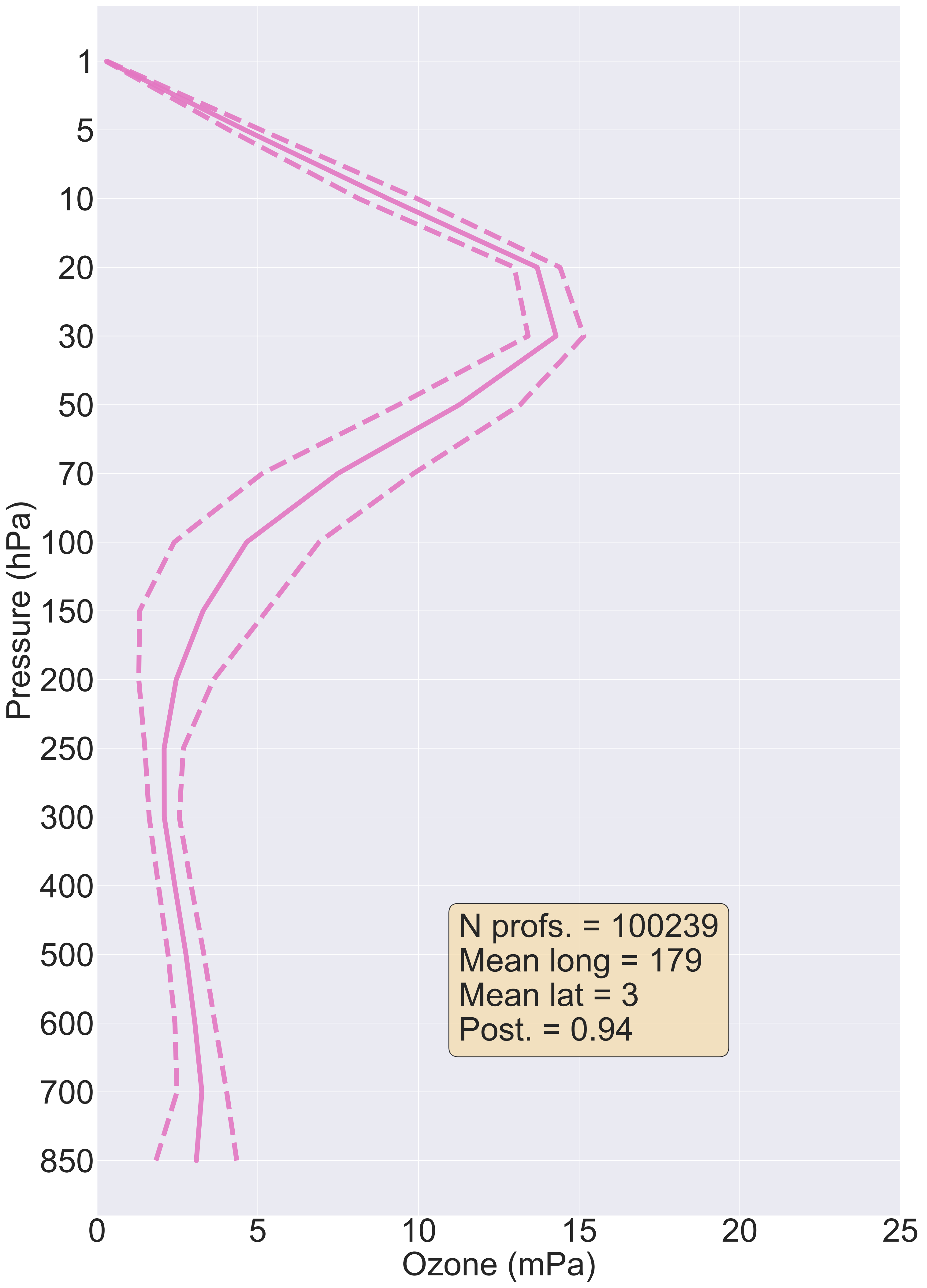
Class = 4
