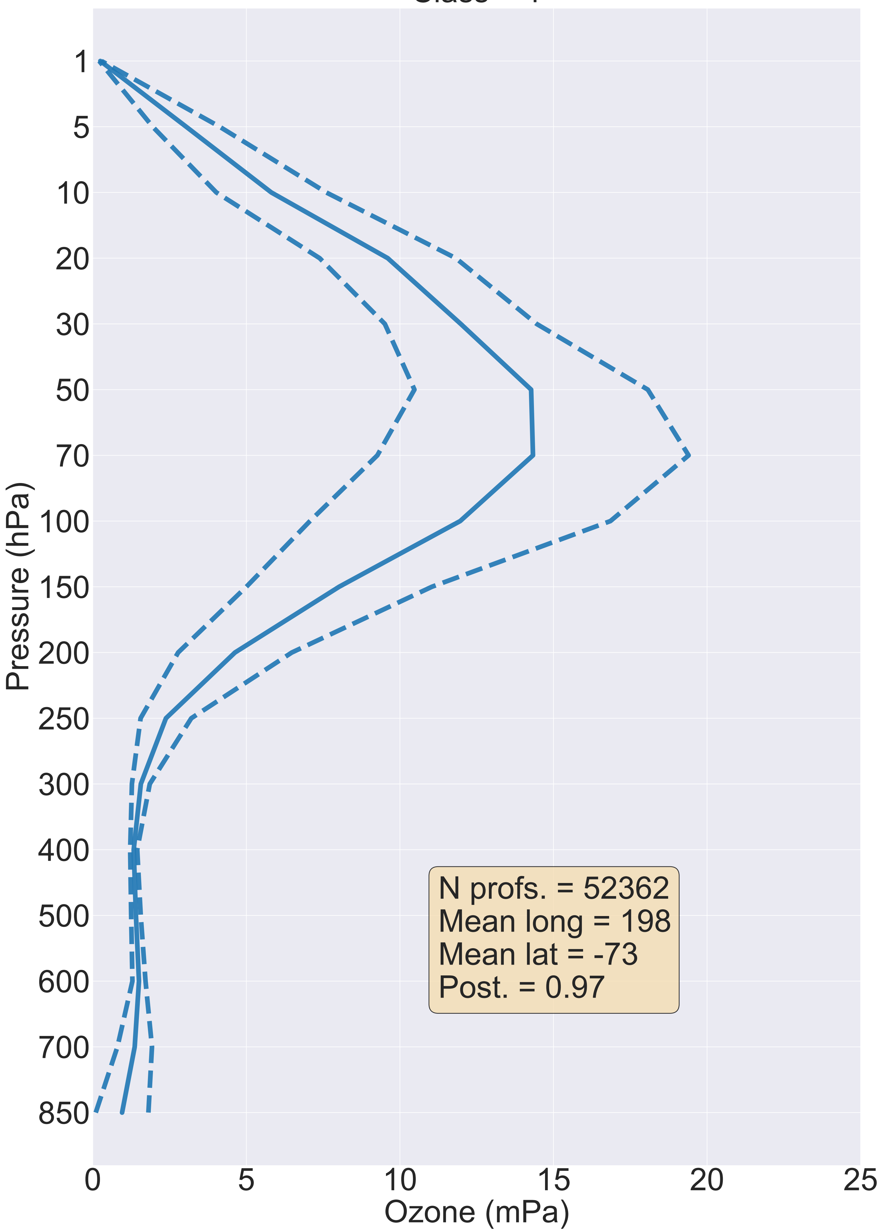
Class = 1
