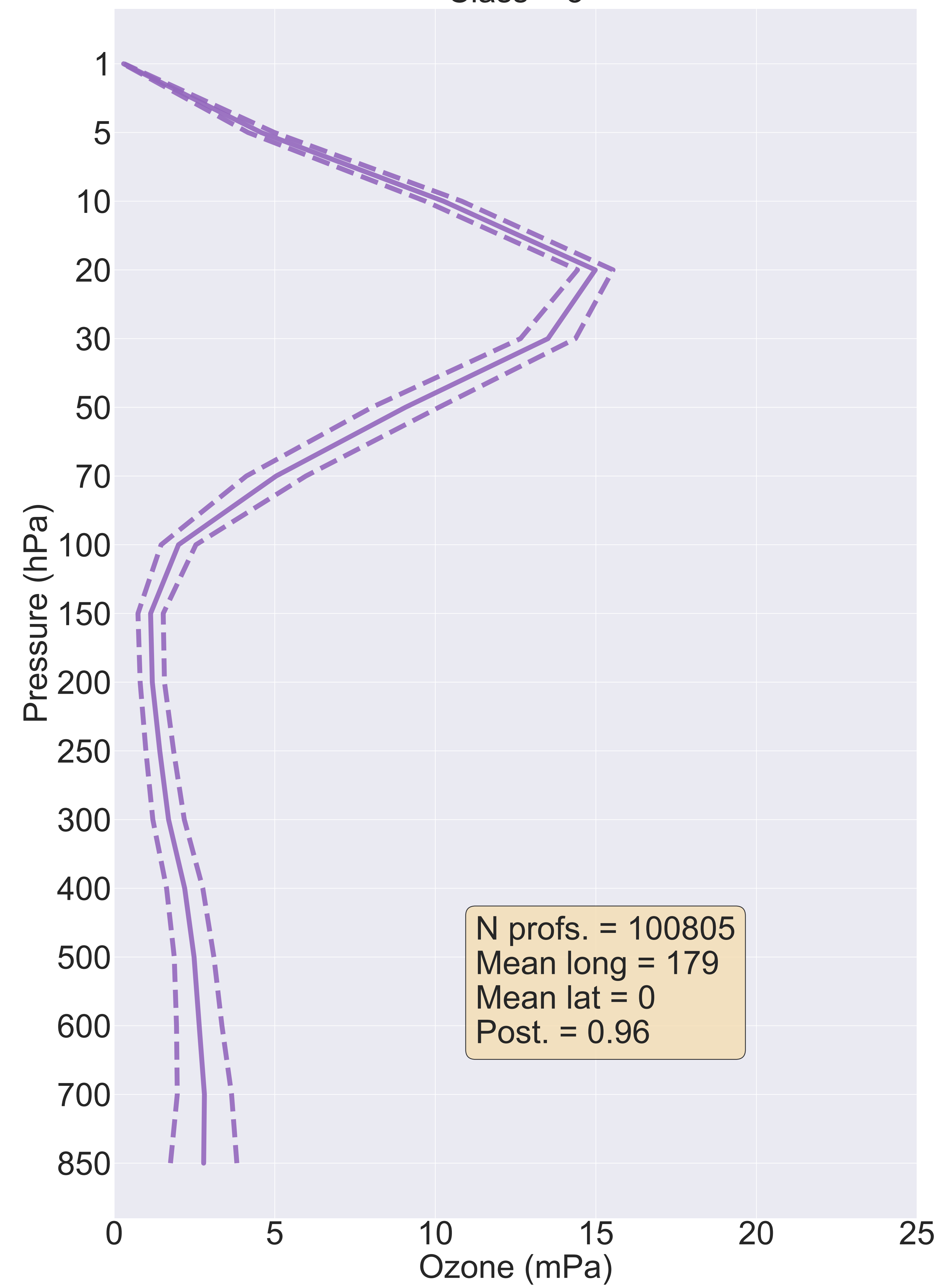
Class = 3
