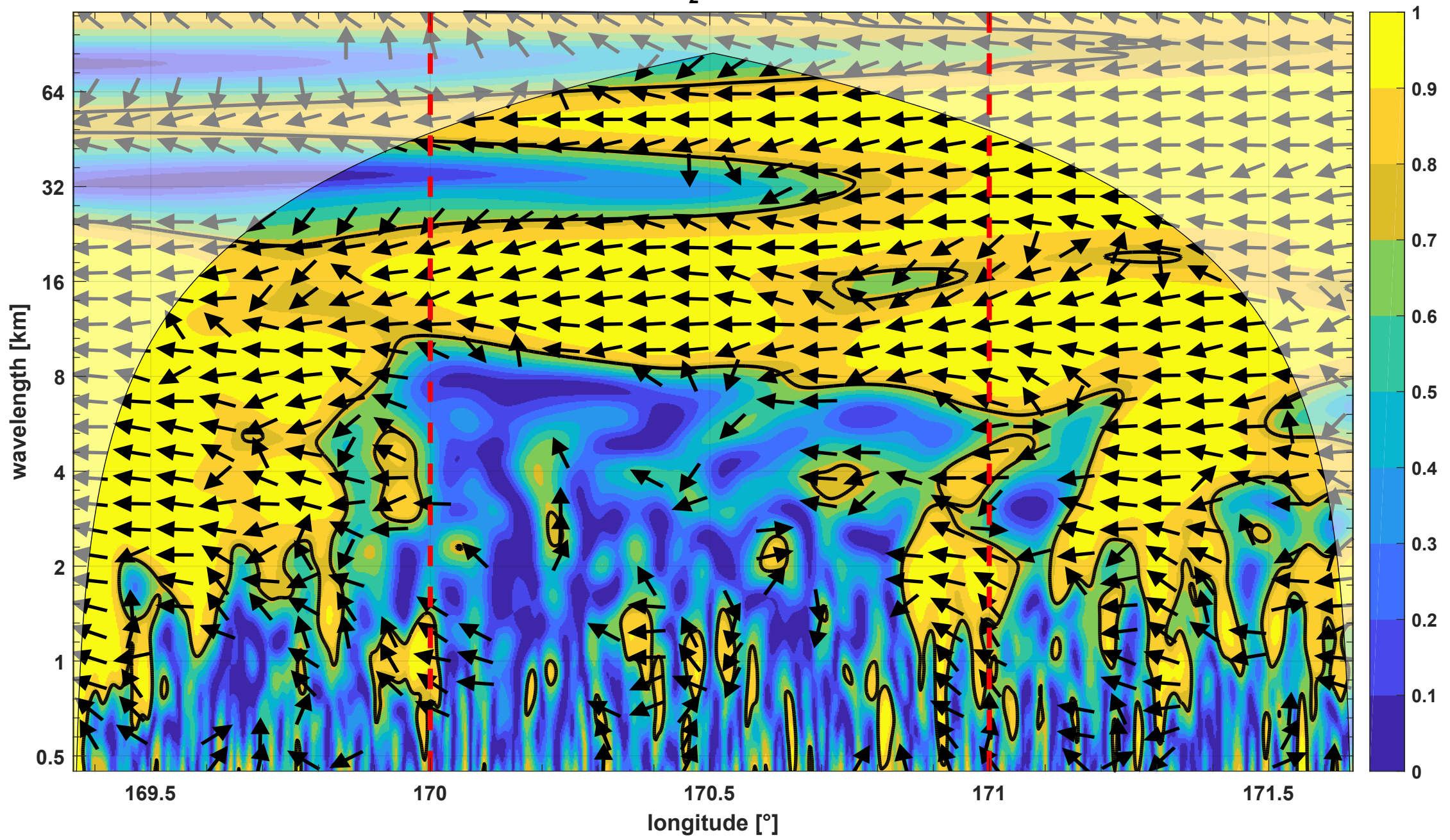
wavelet coherence: N 2 O - potential temperature
