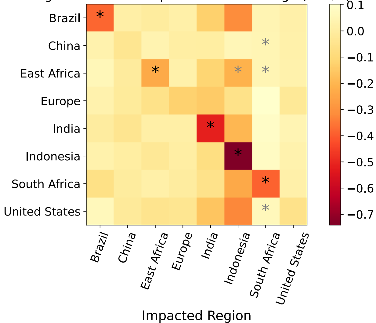
Regional-Mean Precipitation Rate Change (mm/d)
