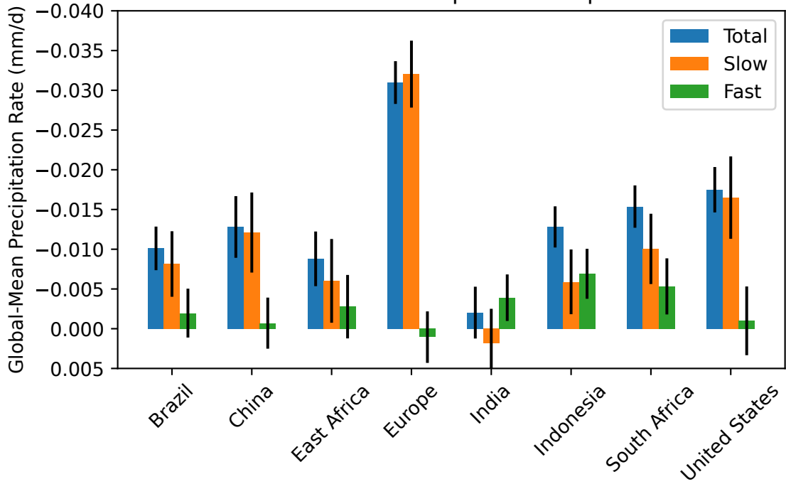
Global-Mean Precipitation Response
