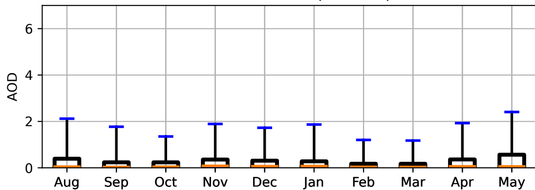
(c) NM - Aerosol optical depth
