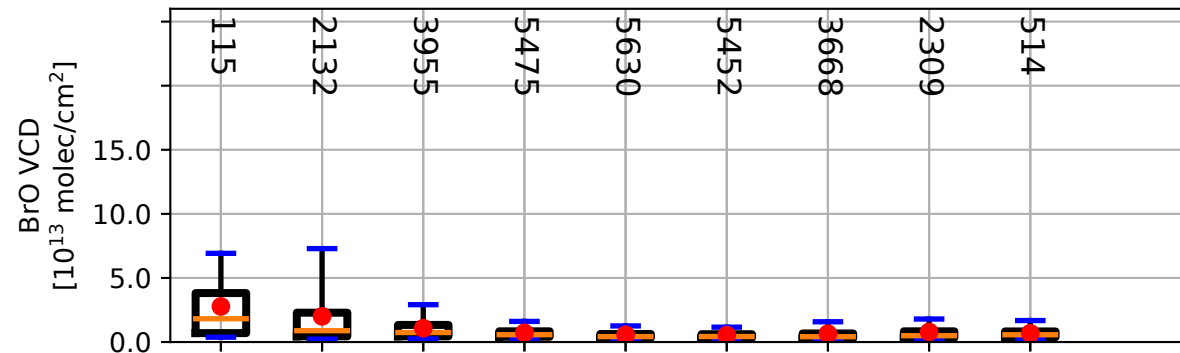
(b) AH - BrO vertical column density
