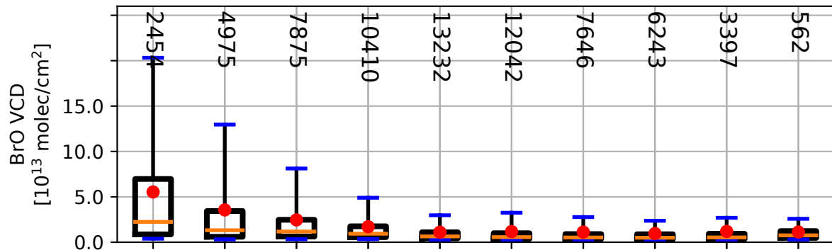
(a) NM - BrO vertical column density
