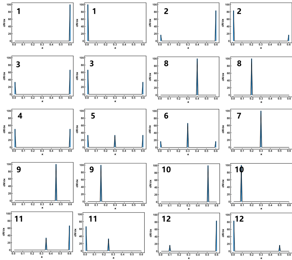
Figure S3. \kappa -PDFs for the 12 populations in the diagram for the particle-to-particle heterogeneity in aerosol hygroscopicity.
