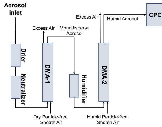
Figure S2. Schematic structure of the H-TDMA
