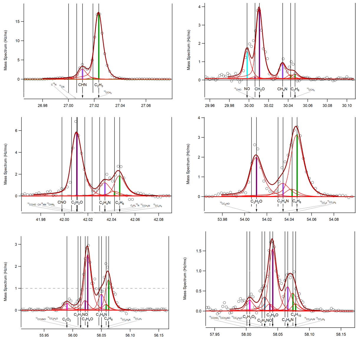
Figure S14. High-resolution mass spectra at dominant \text{C}_x\text{H}_y\text{N}_z m/z ratios taken at T_v = 600 °C.
