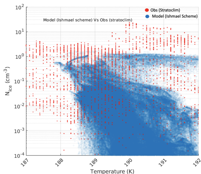
Figure 10. Simulated (blue) and observed (red dots) N_{\text{ice}} versus temperature at 17 km using the ISHMAEL scheme.
