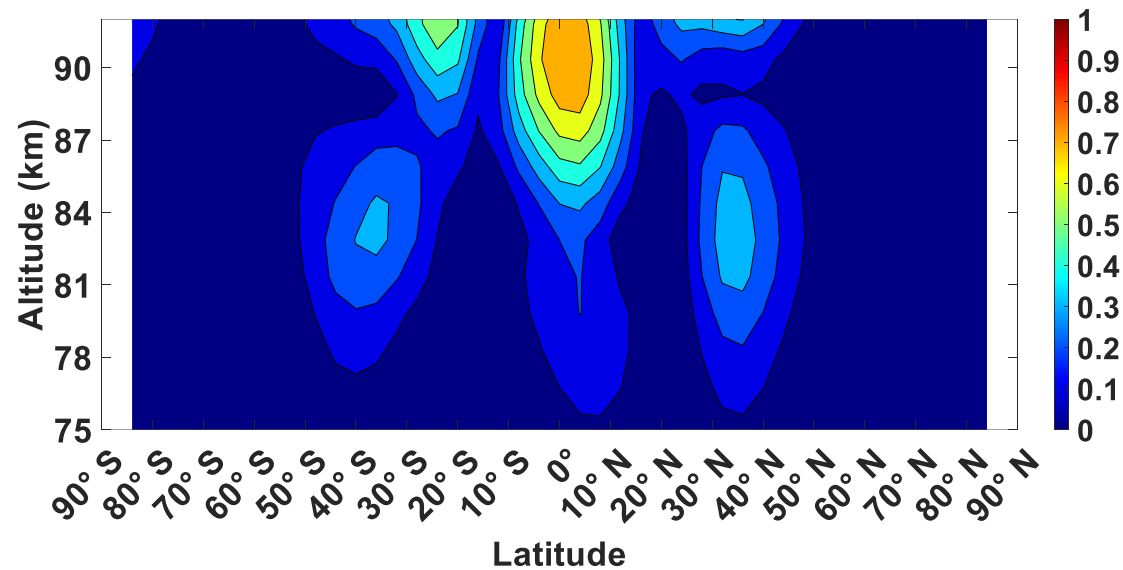
(c) DW1 amplitude of zonal advection term in March (ppm/day)
