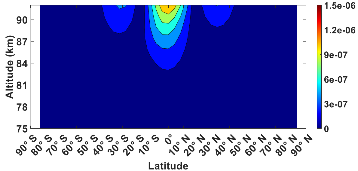
(f) DW1 amplitude of molecular diffusion term in March (ppm/day)
