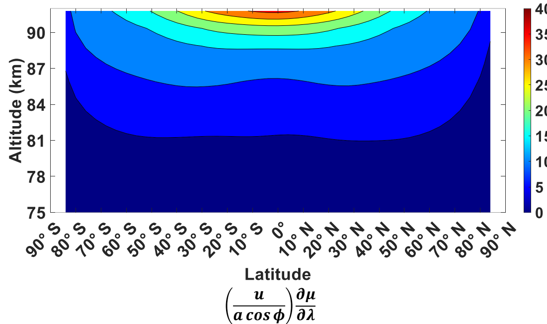
(c) DW1 amplitude of zonal advection term in March (ppm/day)
