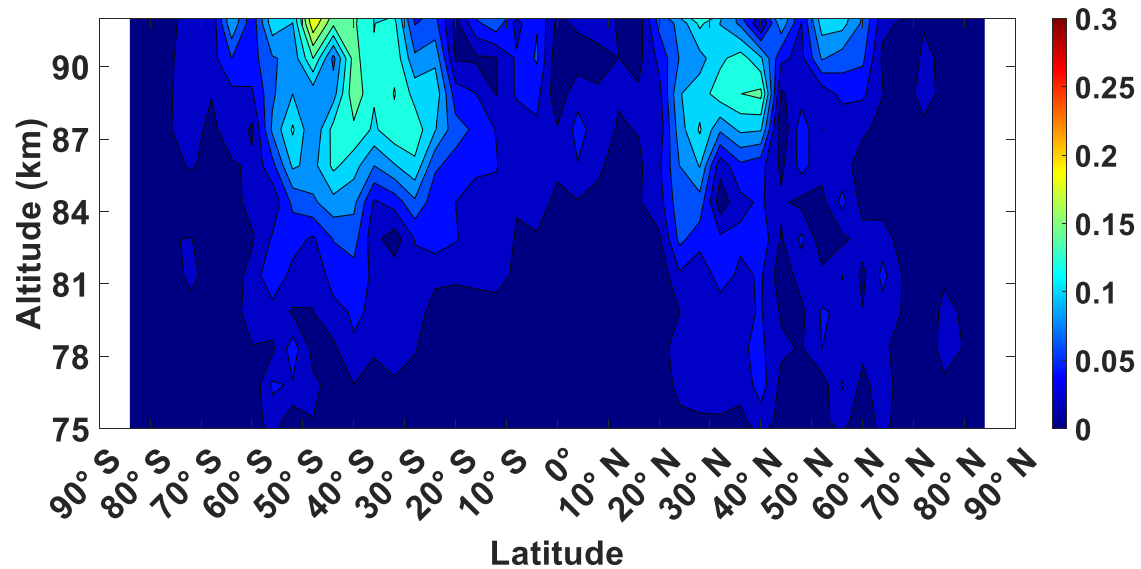
(e) DW1 amplitude of eddy diffusion term in March (ppm/day)
