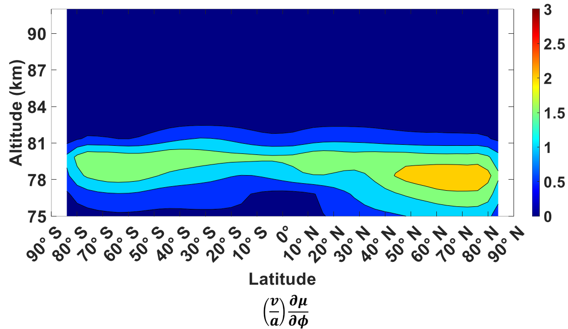
(d) DW1 amplitude of meridional advection term in March (ppm/day)
