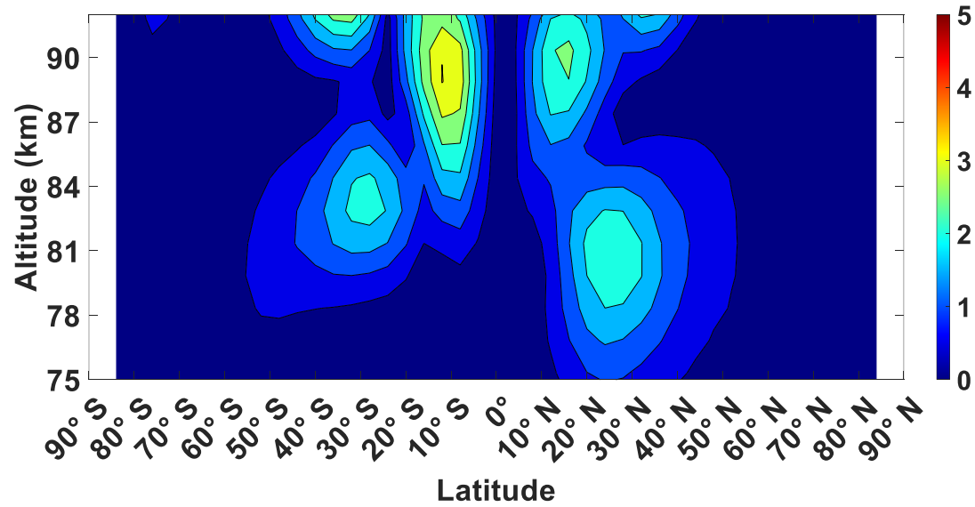
(d) DW1 amplitude of meridional advection term in March (ppm/day)
