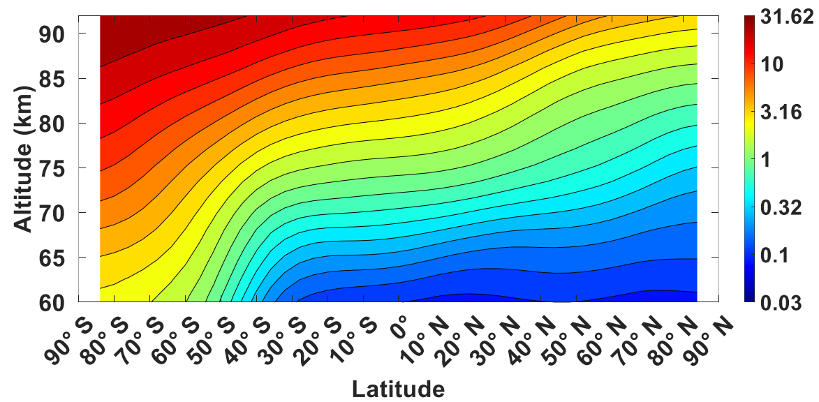
(d) SD-WACCM-X daily-mean zonal-mean CO in December (ppm)
