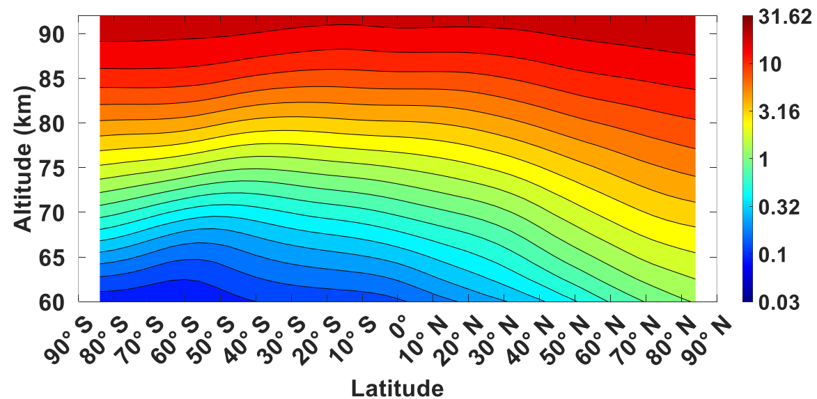
(b) SD-WACCM-X daily-mean zonal-mean CO in September (ppm)
