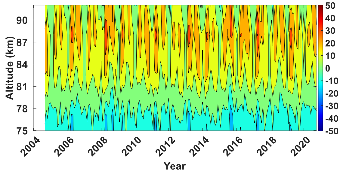
(b) MLS T (1,1) perturbation (K)
