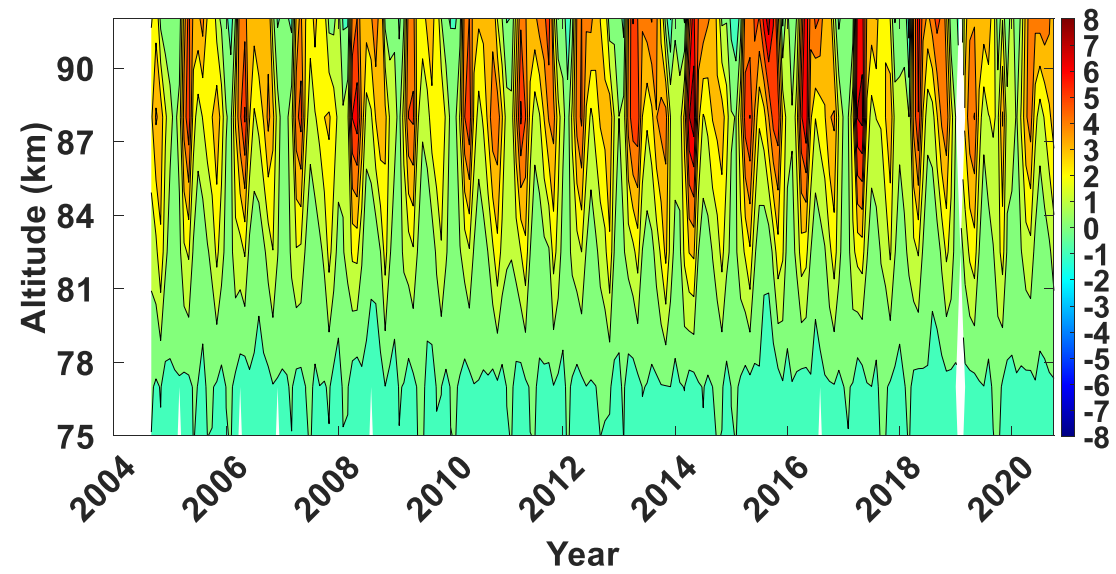
(c) Reconstructed MLS CO (1,1) perturbation (ppm)
