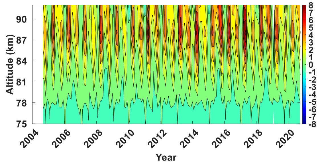
(a) MLS CO (1,1) perturbation (ppm)
