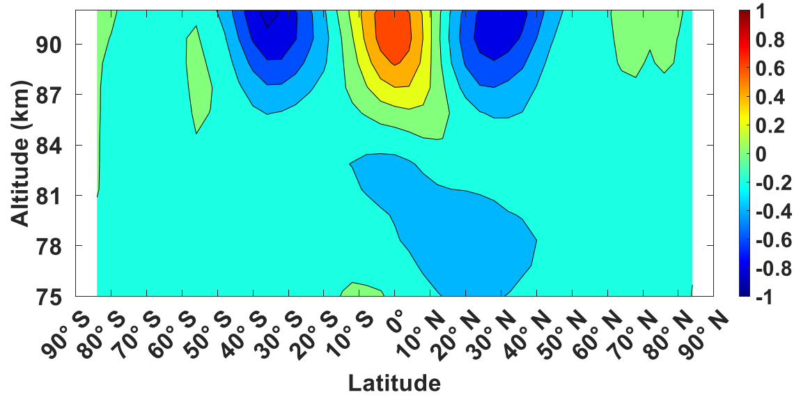
(c) Original SD-WACCM-X CO - reconstructed CO in March (ppm)
