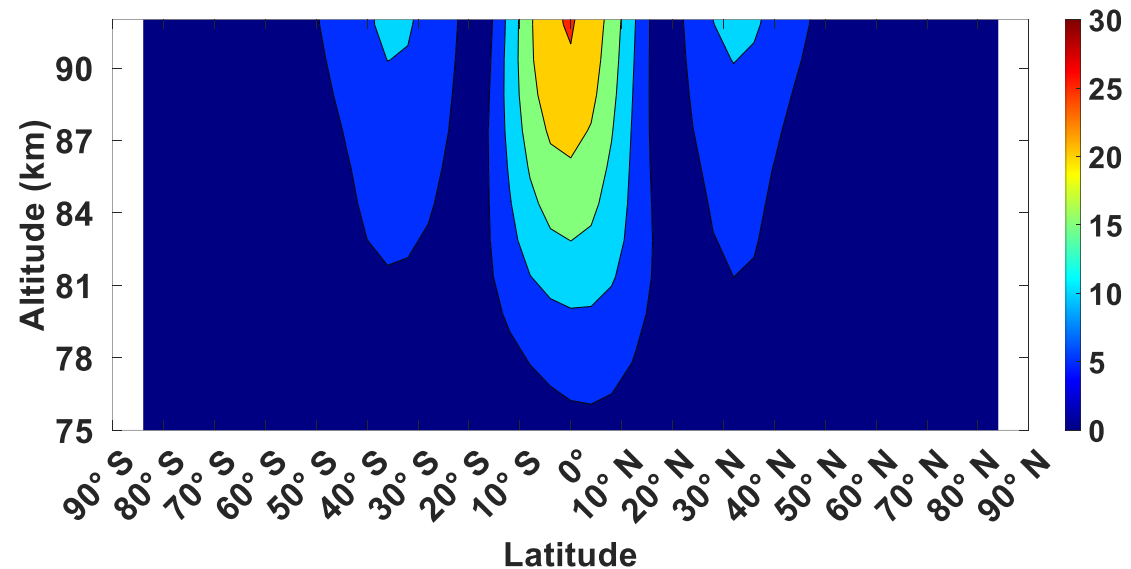
(b) DW1 amplitude of vertical advection term in March (ppm/day)
