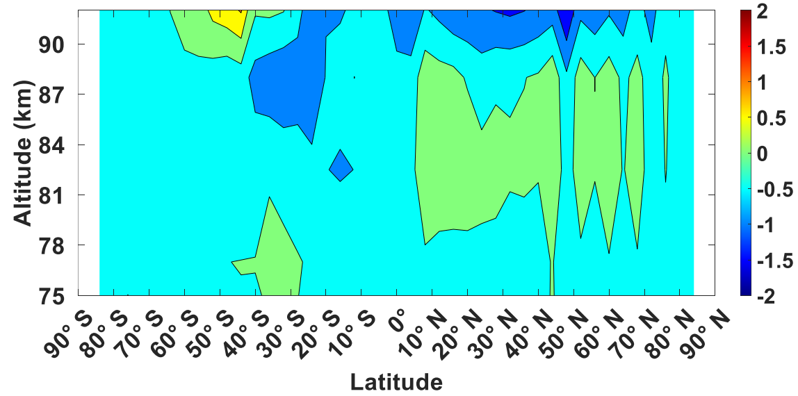
(d) Original MLS CO - reconstructed MLS CO in March (ppm)
