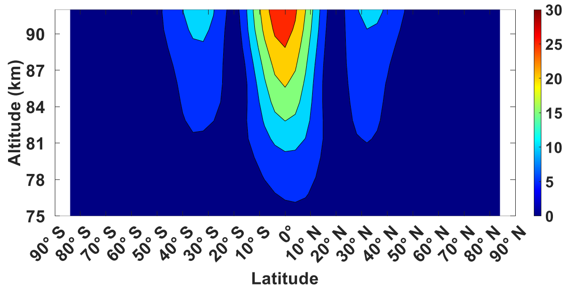
(a) DW1 amplitude of time-derivative term in March (ppm/day)
