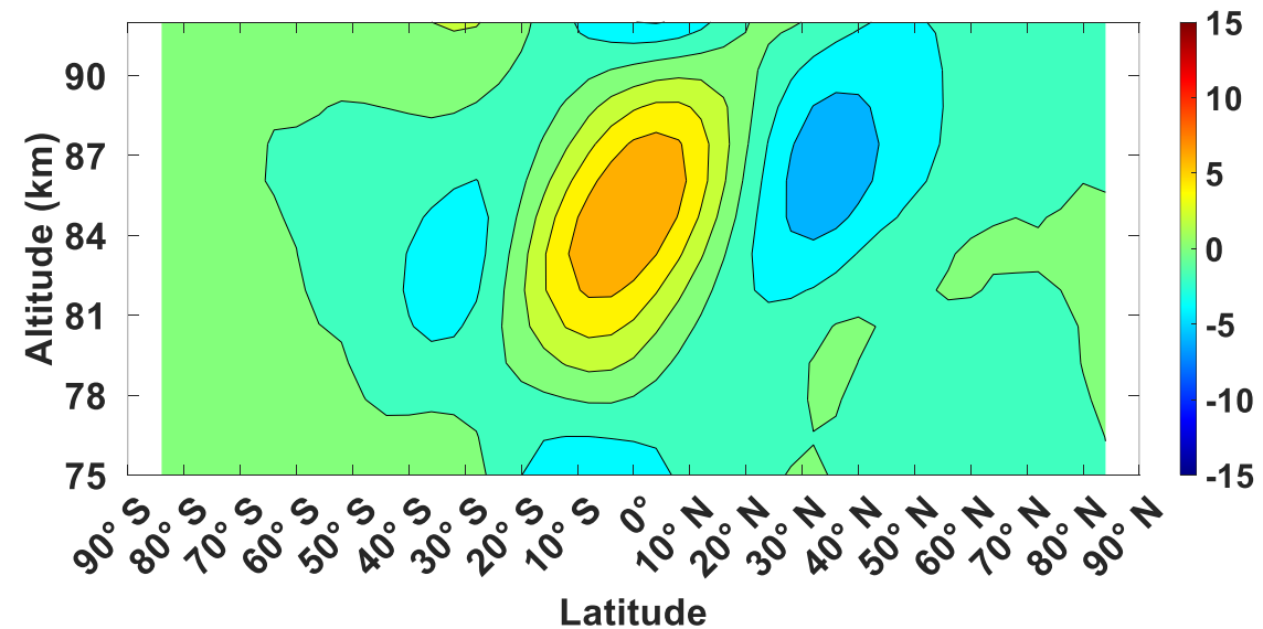
(f) SD-WACCM-X T 2AM-2PM in June (K)
