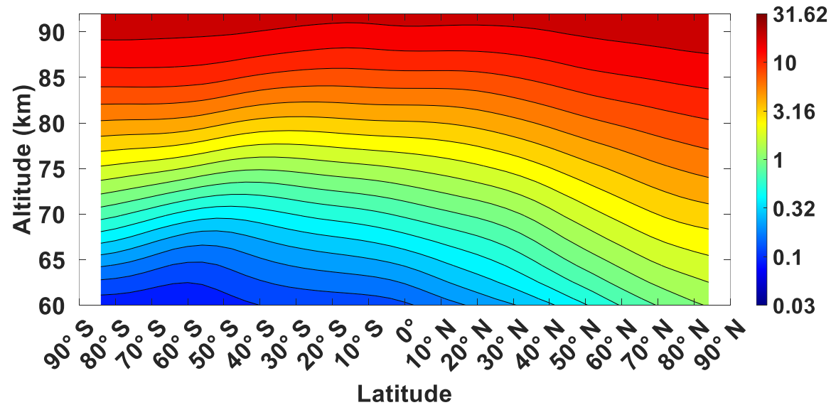
(b) SD-WACCM-X daily-mean zonal-mean CO in March (ppm)
