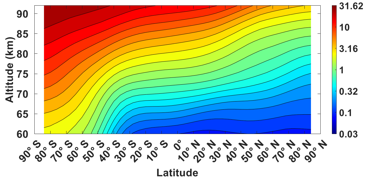
(d) SD-WACCM-X daily-mean zonal-mean CO in June (ppm)
