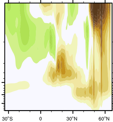
(e) ARISE-SAI-1.5
