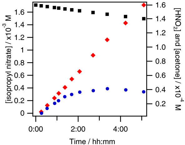
(b) Isopropyl nitrate photolysis (Exp. 4)
