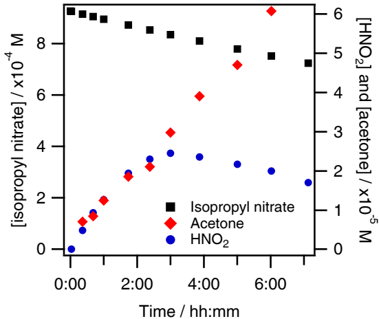
(a) Isopropyl nitrate photolysis (Exp. 2)
