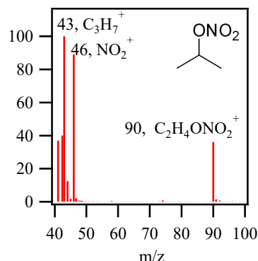
Isopropyl nitrate
