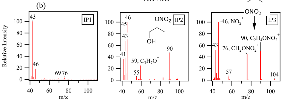
Mass Spectra: Peak at 10.8 min
