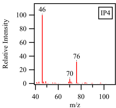
Mass Spectra: Peak at 18.2 min
