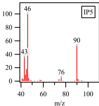
Mass Spectra: Peak at 19.0 min
