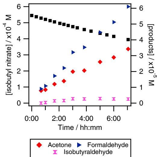
(b) Isobutyl nitrate photolysis
