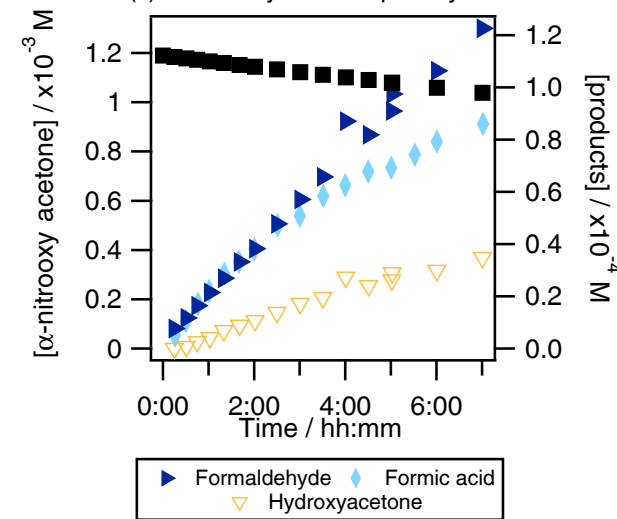
(c) \alpha -Nitrooxy acetone photolysis
