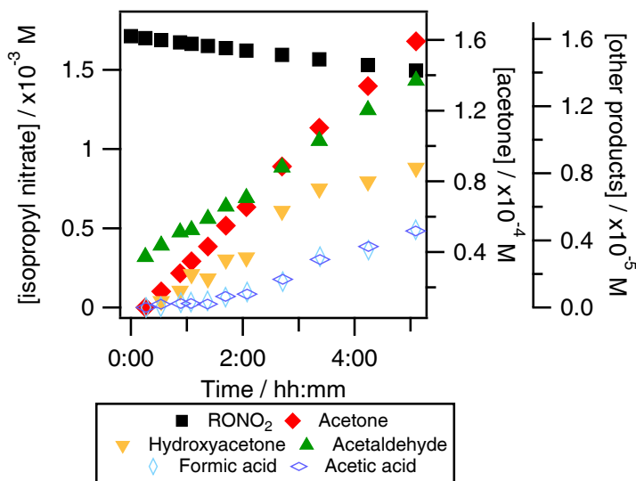
(a) Isopropyl nitrate photolysis
