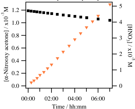
(c) \alpha -Nitrooxy acetone photolysis
