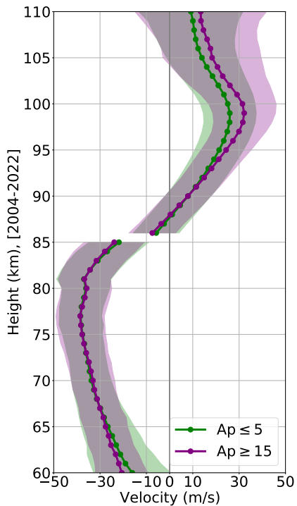
(a) Zonal wind
