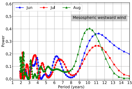
(b) ML LS periods westward [1990 - 2022]
