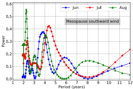
(c) ML LS periods southward [2004 - 2022]
