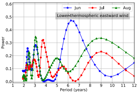
(a) ML LS periods eastward [2004 - 2022]
