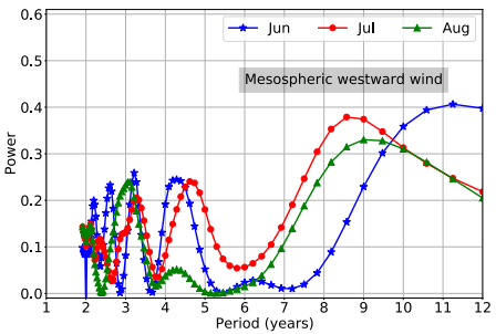
(e) HL LS periods westward [2004 - 2022]
