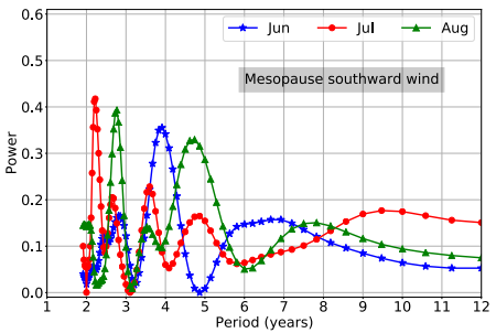
(f) HL LS periods southward [2004 - 2022]
