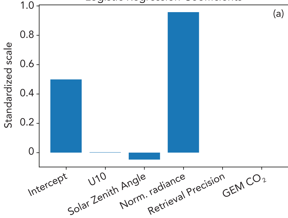
Logistic Regression Coefficients
