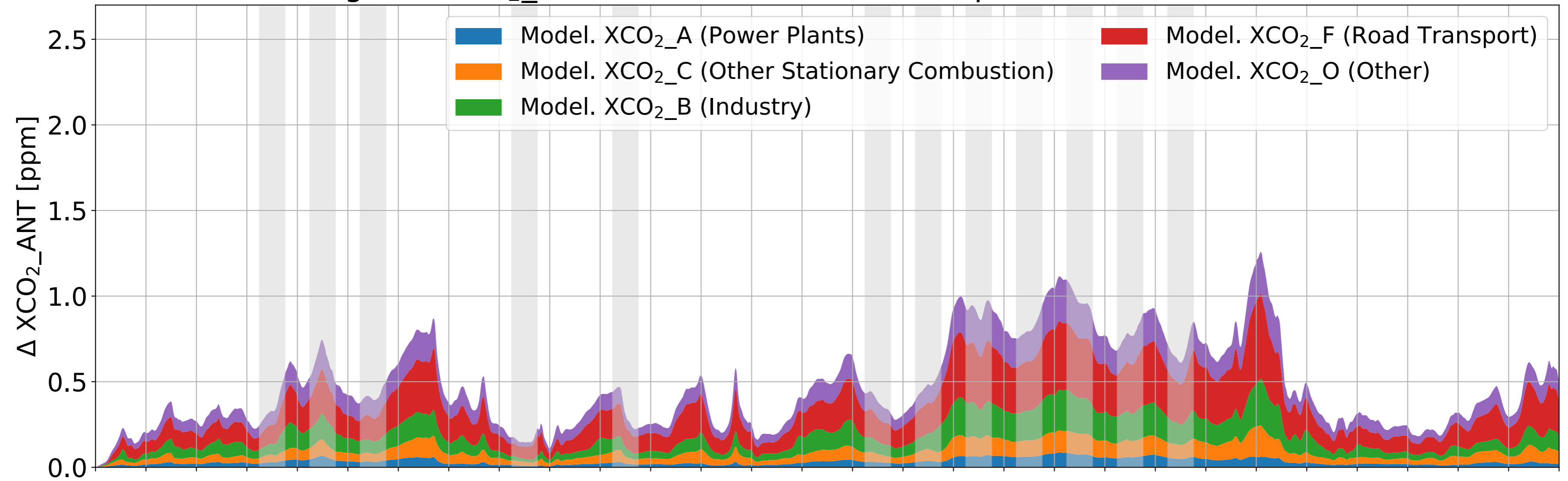
(a) Model. Averaged \Delta XCO_2\_ANT from different emission processes in and around Munich (D03)
