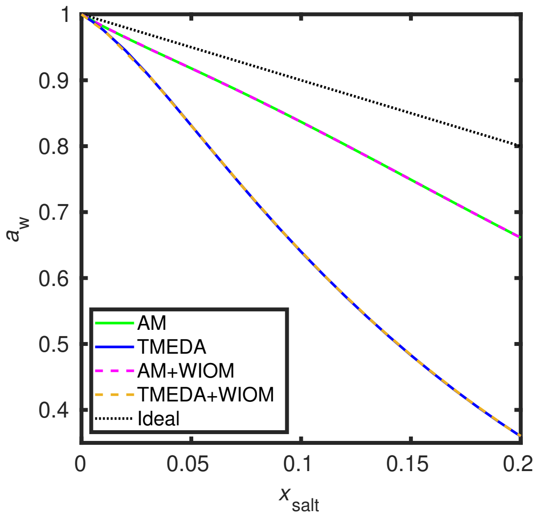
Figure S13: COSMO therm -predicted water activities a_w in methylsulfonate solutions with and without WIOM. The amount of WIOM at each salt mole fraction is mole fraction of WIOM at LLE computed using COSMO therm .
