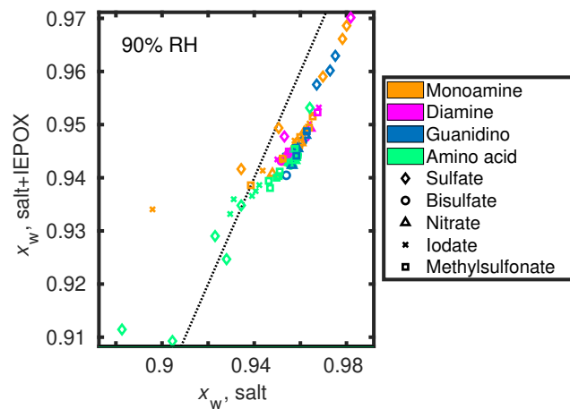
Figure S11: COSMO therm -derived equilibrium water contents ( x_w in mole fraction) in 90% RH at 298.15 K. The black dotted lines represent the 1:1 line.
