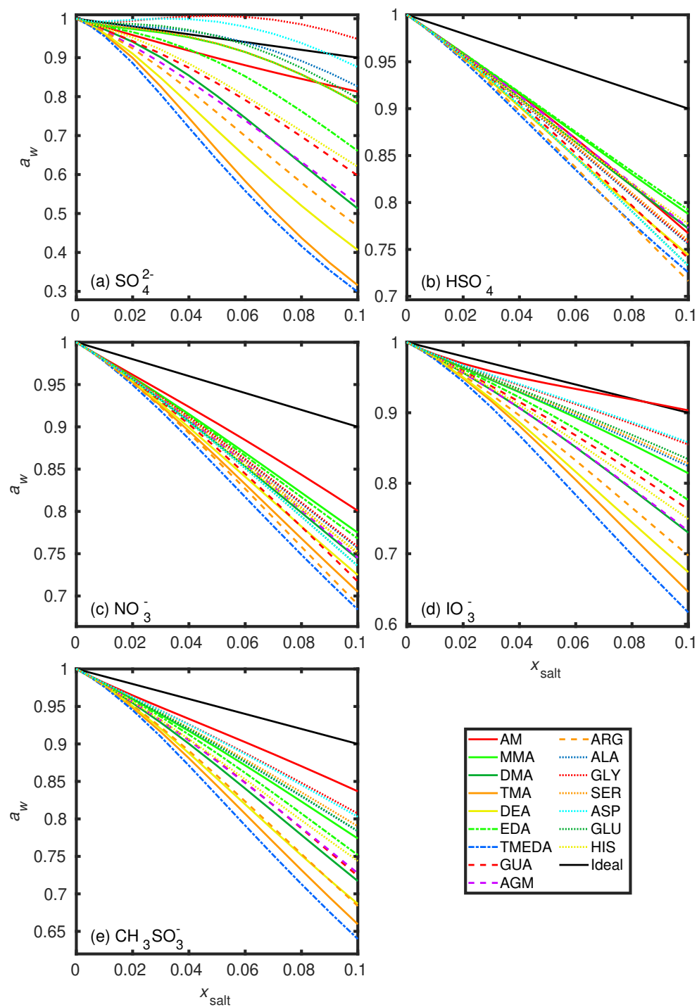
Figure S8: COSMOtherm-derived water activities ( a_w ) in (a) sulfates, (b) bisulfates, (c) nitrates, (d) iodates and (e) methylsulfonates at 298.15 K. Activities were calculated in 0.01 intervals of salt mole fraction ( x_{\text{salt}} ) and plotted as lines for clarity.
