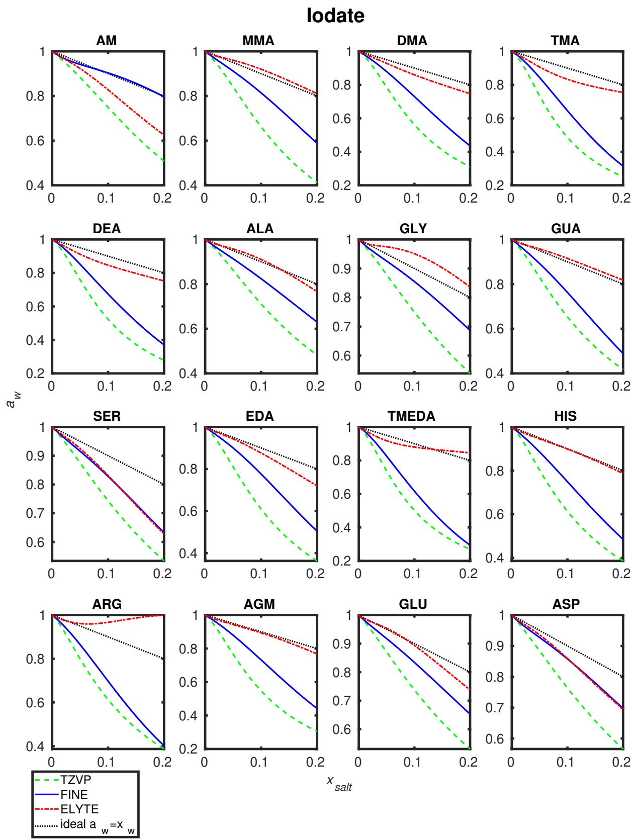
Figure S5: Comparison between COSMOtherm parametrizations in aqueous iodate salt solutions at 298.15 K.
