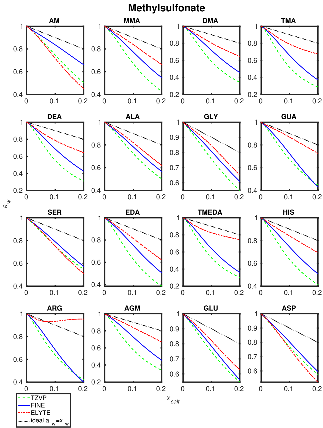
Figure S6: Comparison between COSMO therm parametrizations in aqueous methylsulfonate salt solutions at 298.15 K.
