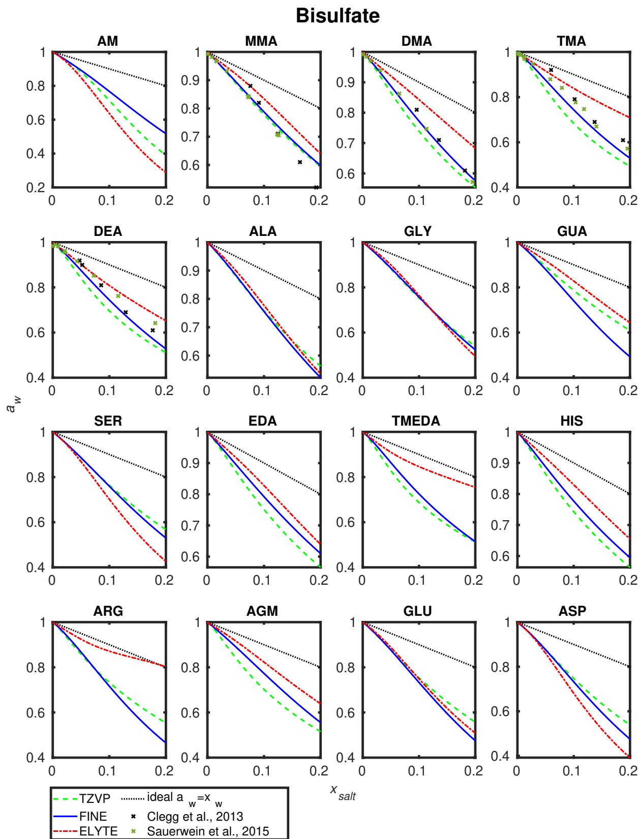
Figure S3: Comparison between experiments S2,S3 and different COSMOtherm parametrizations in aqueous bisulfate salt solutions at 298.15 K.
