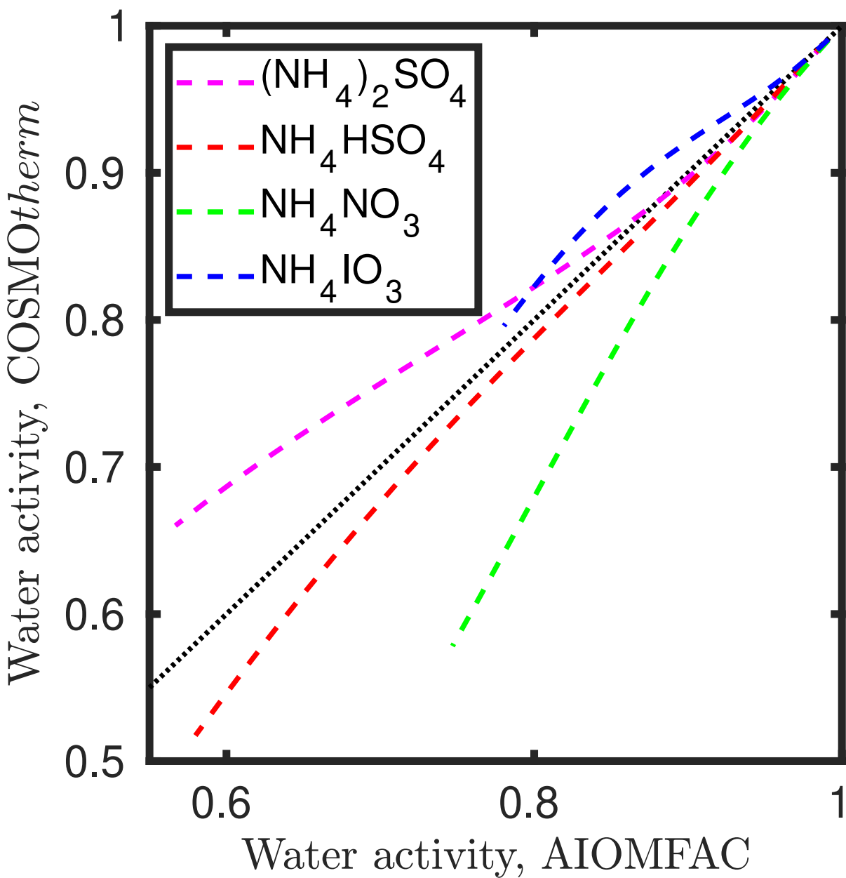
Figure S1: Comparison between COSMOTHERM- and AIOMFAC S1 -derived water activities in ammonium salts at 298.15 K. Water activities were calculated for solutions with salt mole fractions from 0 to 0.2. The black dotted line shows the 1:1 line.
