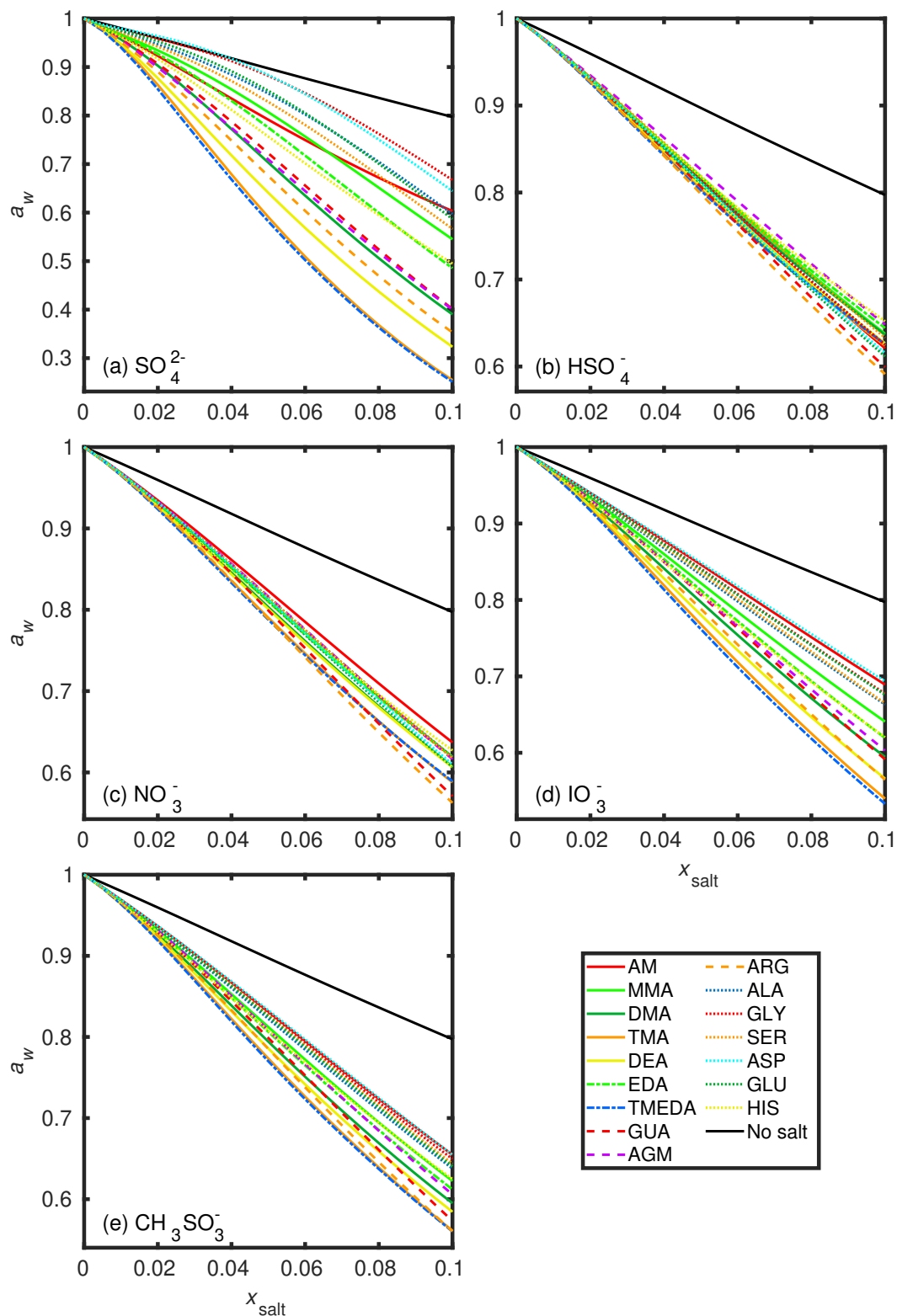
Figure S12: COSMO therm -derived water activities in (a) sulfate, (b) bisulfate, (c) nitrate, (d) iodate and (e) methylsulfonate in the presence of IEPOX at 298.15 K. The mole fraction of IEPOX is equal to x_{\text{salt}} , the remaining mole fraction is water. "No salt" contains only water and IEPOX with a mole fraction of 2 \times x_{\text{salt}} . Activities were calculated in 0.01 salt mole fraction intervals and plotted as lines for clarity.
