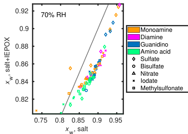
Figure S10: COSMO therm -derived equilibrium water contents ( x_w in mole fraction) in 70% RH at 298.15 K. The black dotted lines represent the 1:1 line.
