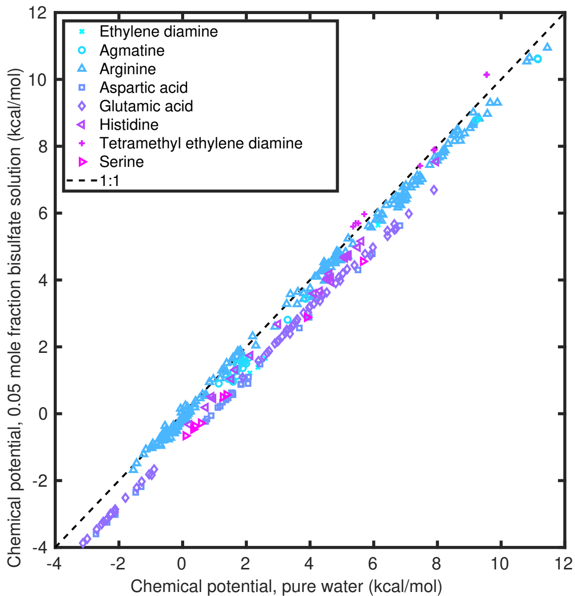
Figure S7: Pseudo-chemical potentials of selected aminium cations in the infinite dilution in water (x-axis) and in 0.05 mole fraction aqueous aminium bisulfate at 298.15 K.
