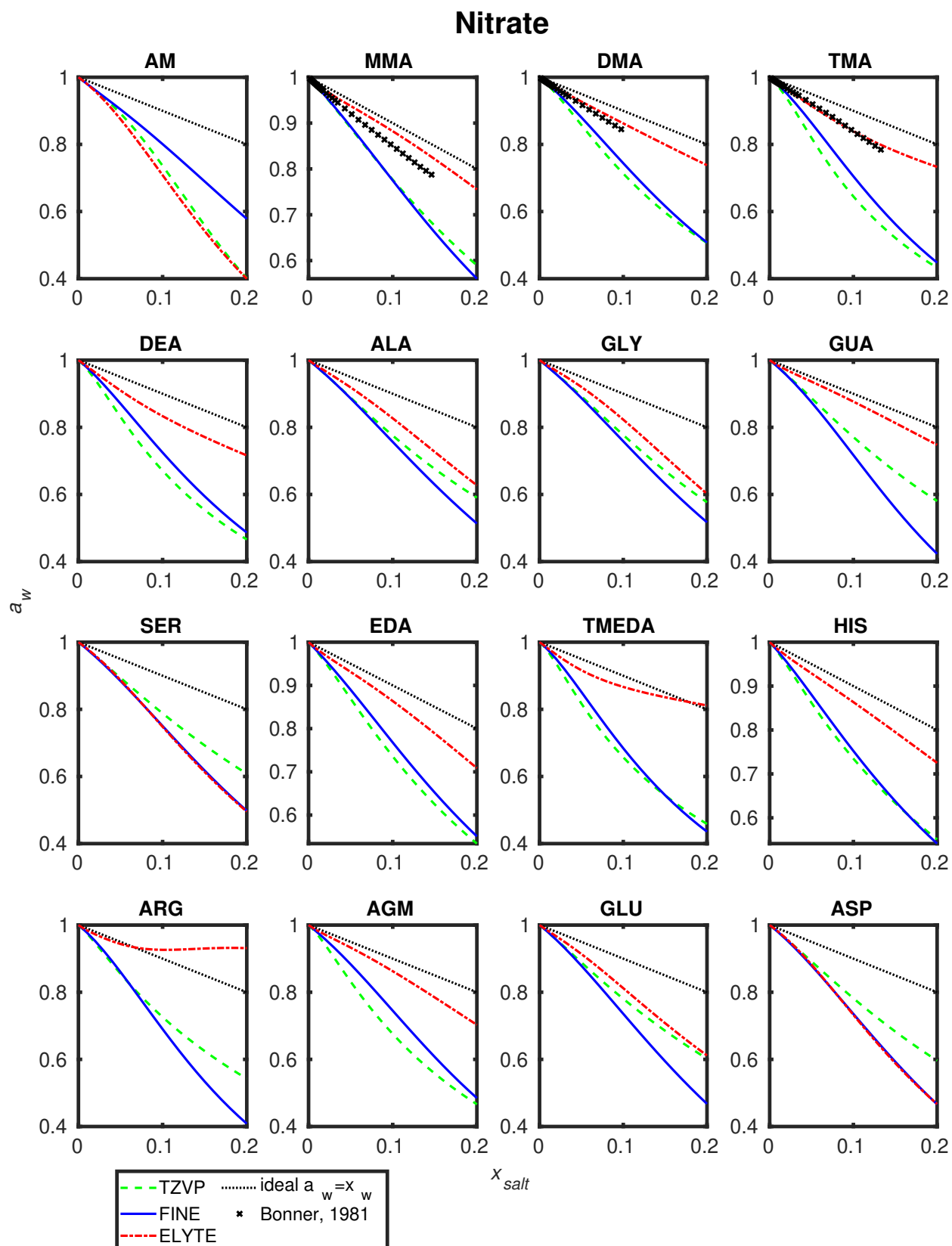
Figure S4: Comparison between COSMOtherm parametrizations in aqueous nitrate salt solutions at 298.15 K. Experimental water activities are calculated from osmotic coefficients of Bonner. S5
