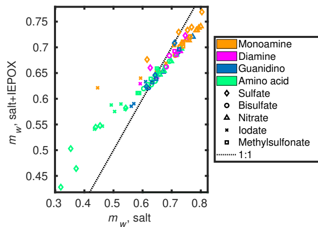
Figure S9: COSMO therm -derived equilibrium water contents ( m_w in mass fraction) in 90% RH at 298.15 K. The black dotted lines represent the 1:1 line.
