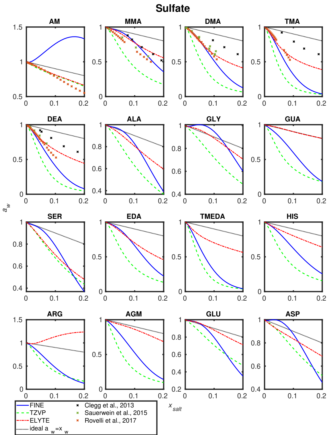
Figure S2: Comparison between experiments S2-S4 and different COSMOtherm parametrizations in aqueous sulfate salt solutions at 298.15 K.
