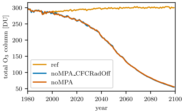
a) Global mean total ozone column (1980-2099)
