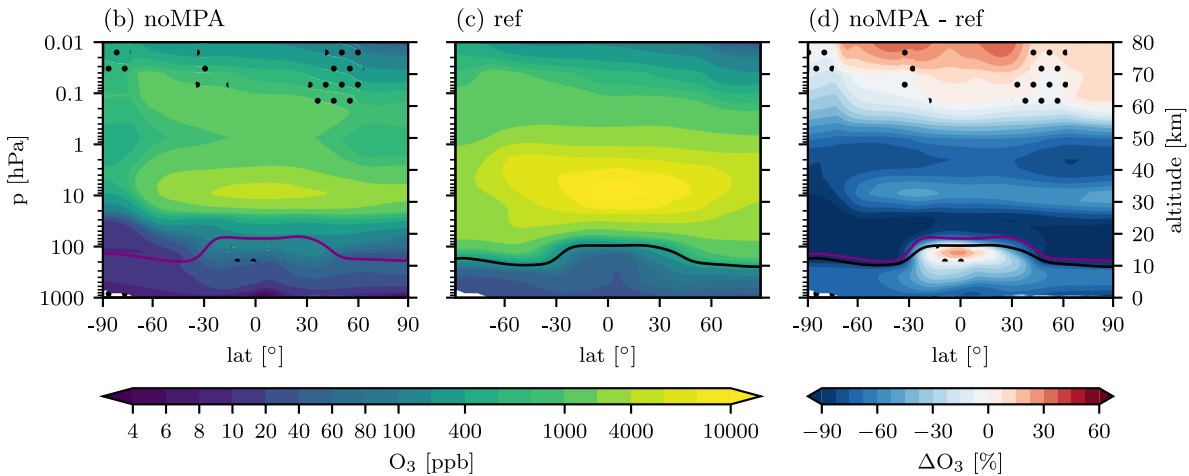
Zonal mean O 3 , JJA 2080-2099
