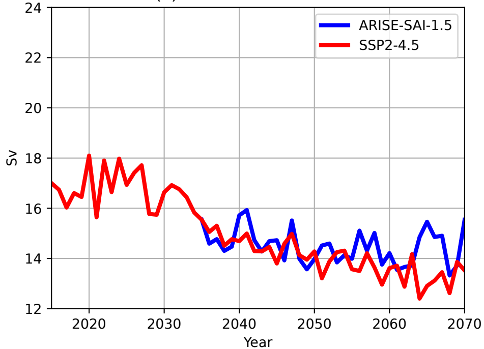
(a) UKESM1 Atlantic MOC
