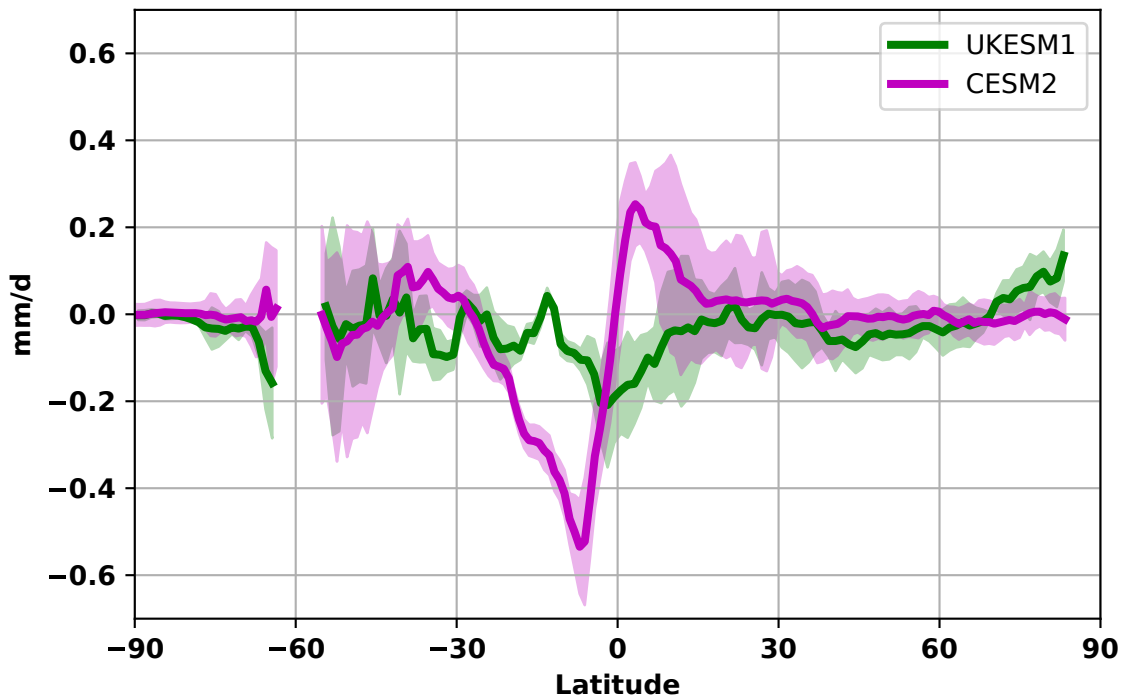
(c) Land precipitation (ARISE-SAI-1.5, DJF, 2050-2069 - reference period)
