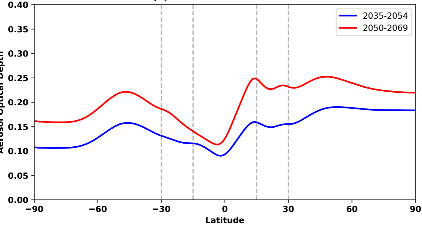
(e) UKESM1 AOD increase
