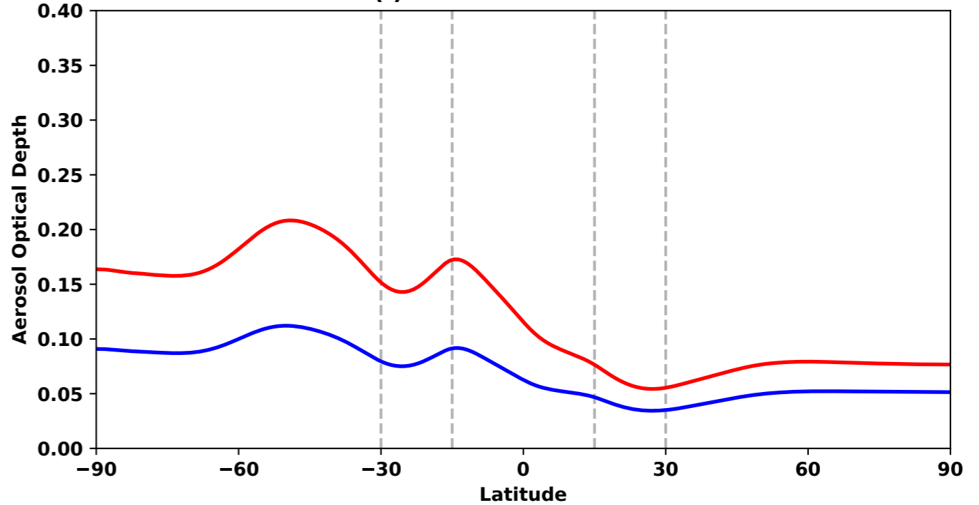
(f) CESM2 AOD increase
