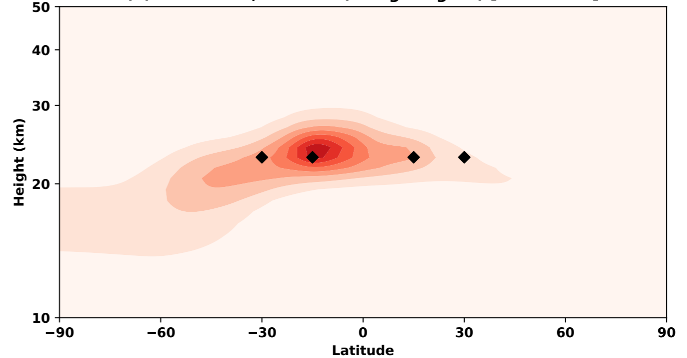
(f) CESM2 AOD increase
