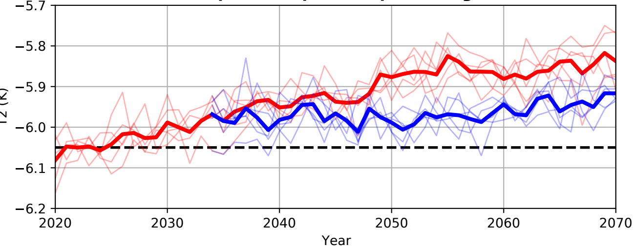
(e) UKESM1 Equator-to-pole temperature gradient (T2)
