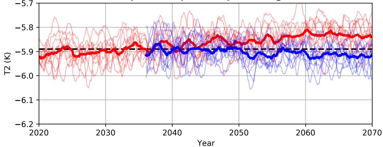
(f) CESM2 Equator-to-pole temperature gradient (T2)
