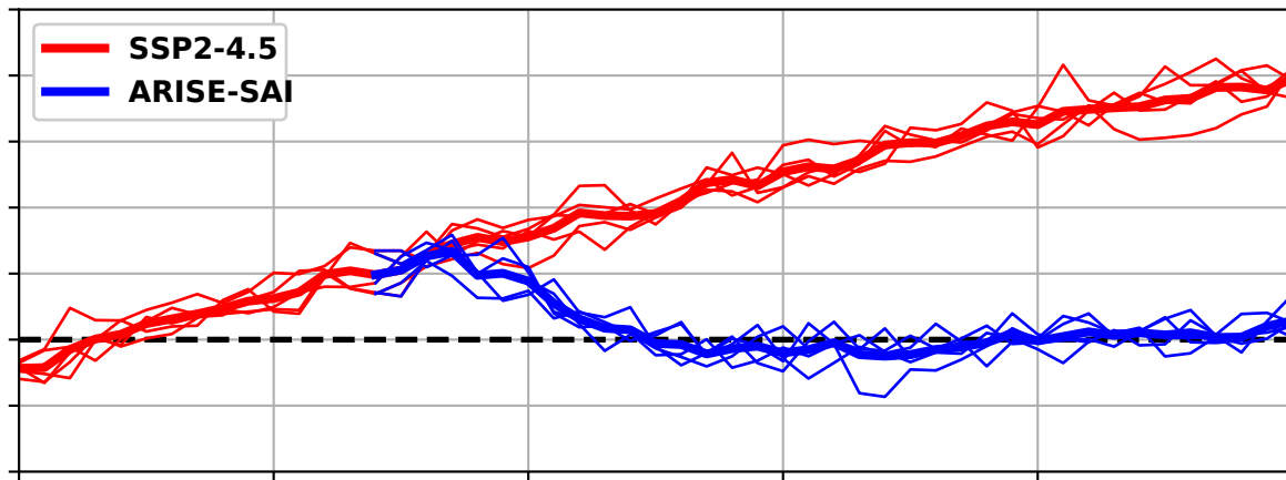
(a) UKESM1 Global mean temperature (T0)
