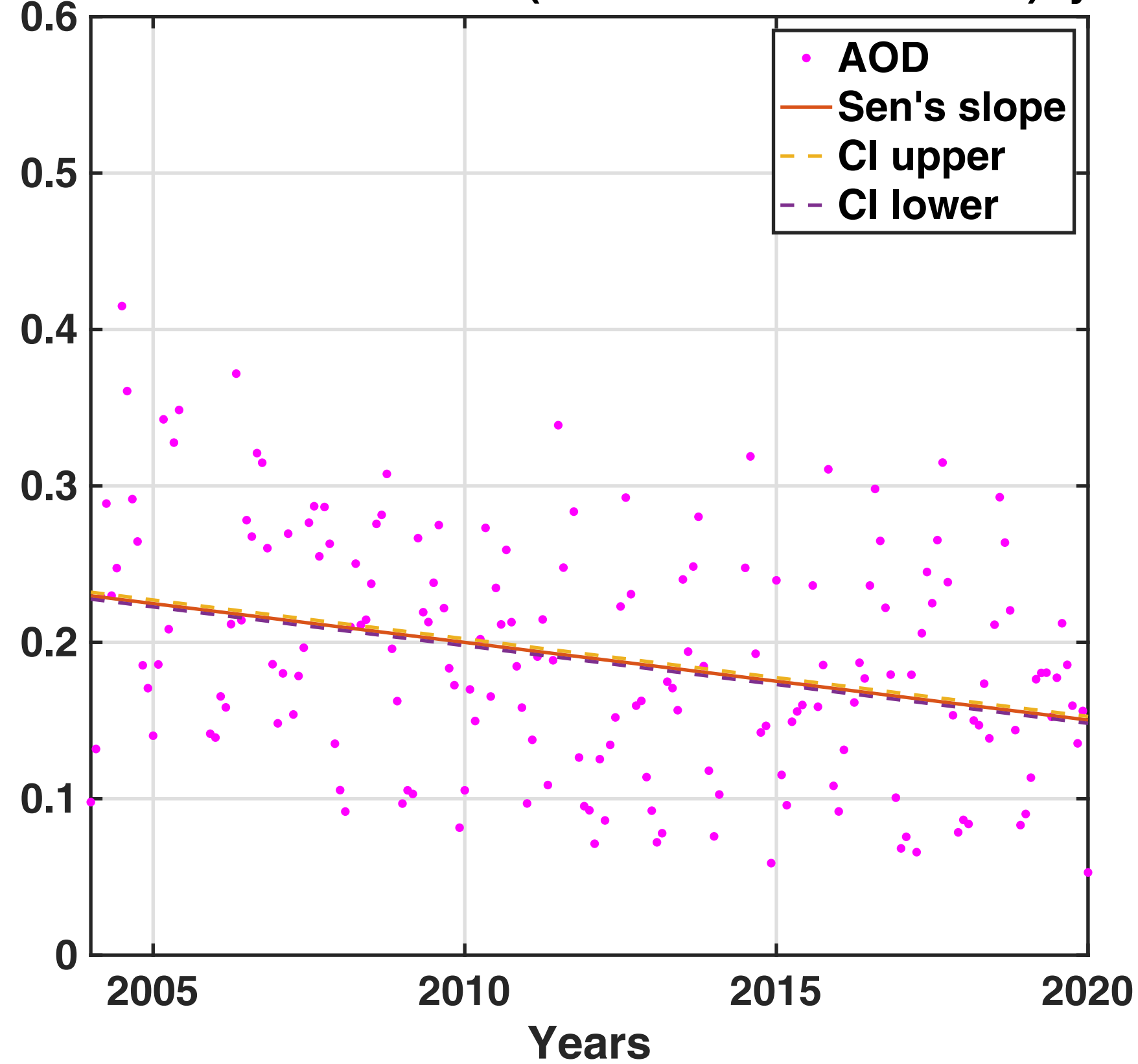
AOD @440nm -0.0054(CI 95%:-0.0060 -0.0038) yr -1
