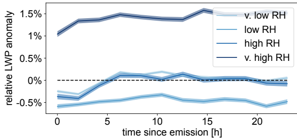
(b) LWP enhancement in RH700 quartiles over time
