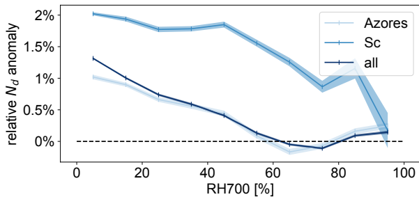
(c) N_d enhancement by RH700 bins
