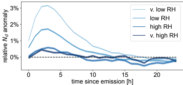
(a) N_d enhancement in RH700 quartiles over time
