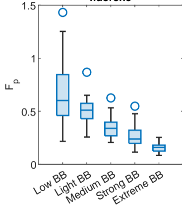
fluorene
