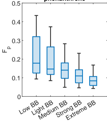
phenanthrene
