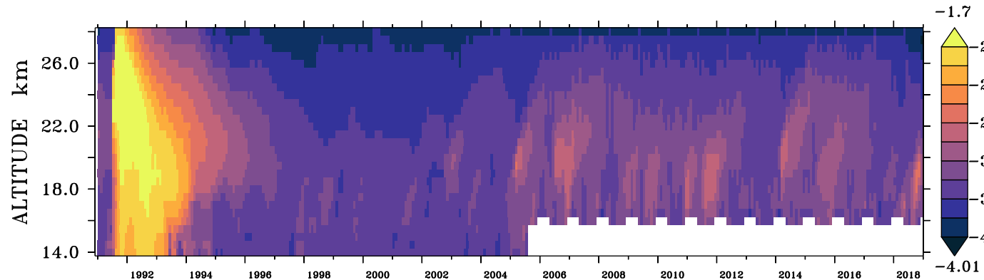
(b) GloSSAC aerosol extinction, 20° S–20° N
