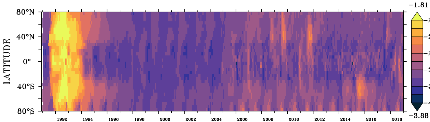
(a) GloSSAC aerosol extinction, 17 km
