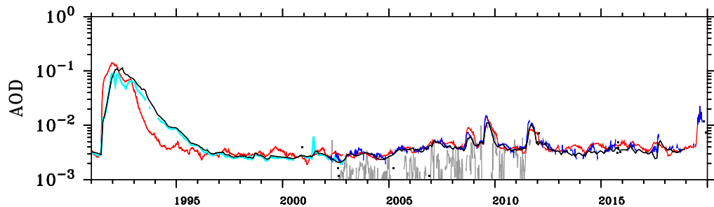
(b) Stratospheric Aerosol Optical Depth 750 nm, 45° N–70° N
