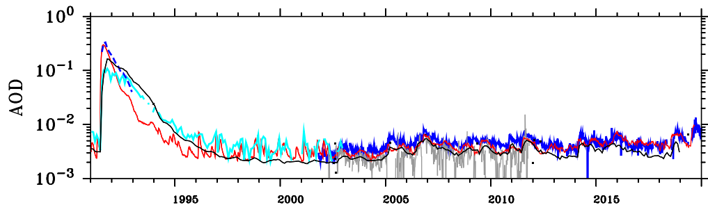
(a) Stratospheric Aerosol Optical Depth 750 nm, 20° S–20° N
