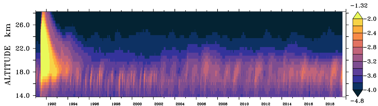
(c) EMAC Simulations of aerosol extinction at 750 nm, 20°S-20°N
