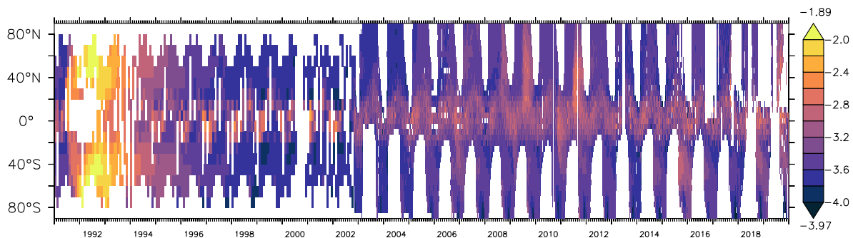
(a) SAGE II / OSIRIS extinction, at 750nm, 1/km, 17 km, log
