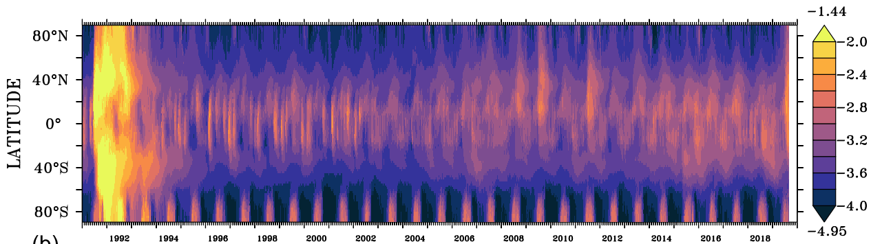
(b) EMAC Simulations of aerosol extinction at 750 nm, 17 km
