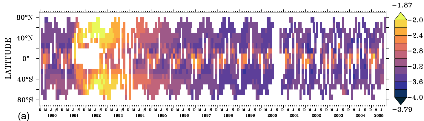
SAGE II 550 nm, 1/km (log), 17 km
