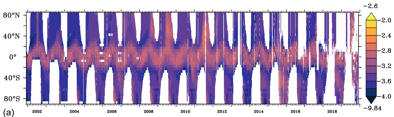
(a) OSIRIS, 750 nm extinction, 1/km (log), 17 km
