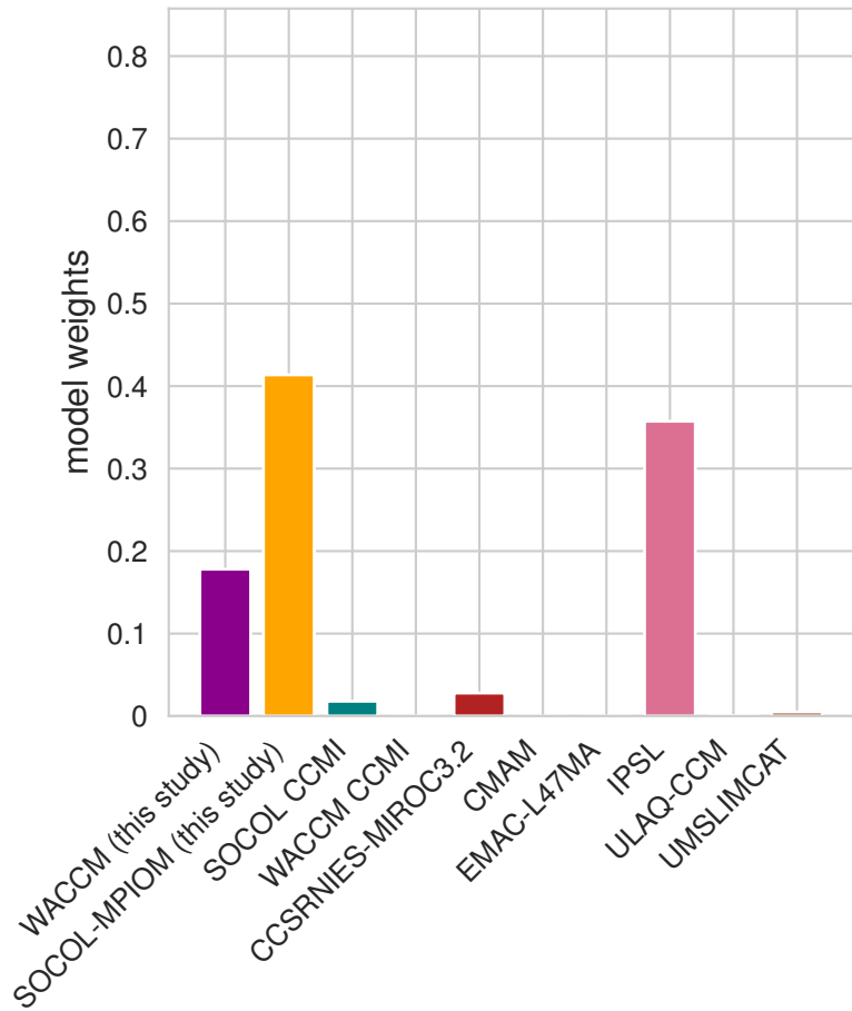
RCP8.5 - CCMI-1
