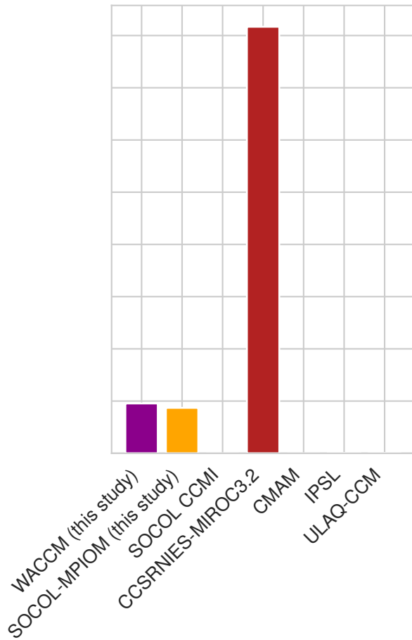
RCP2.6 - CCMI-1
