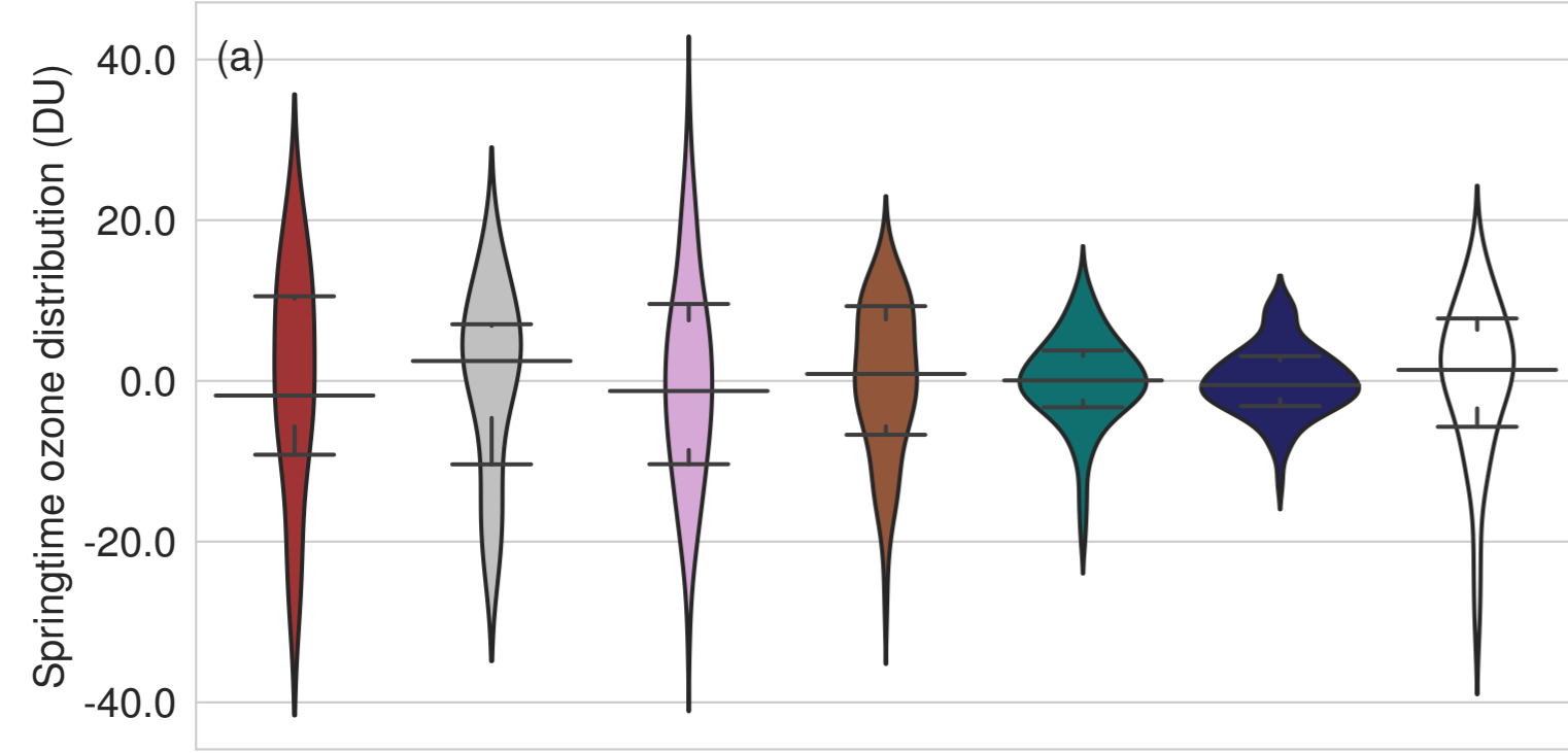
Springtime ozone distribution, 2005-2029
