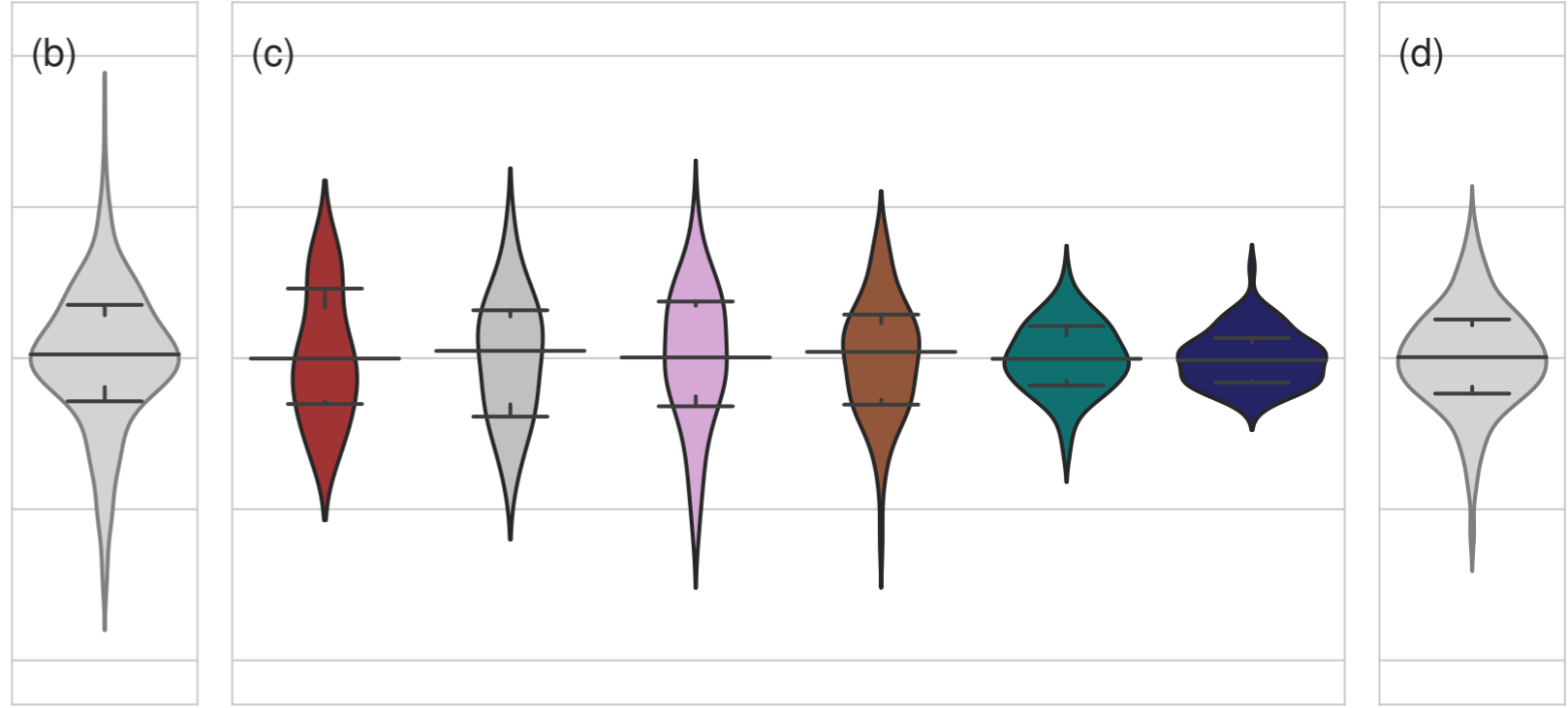
Springtime ozone distribution, 2070-2094
