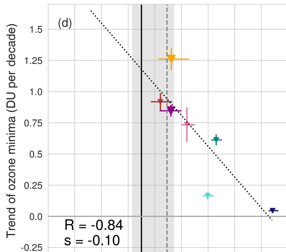
RCP2.6 - CCMI-1
