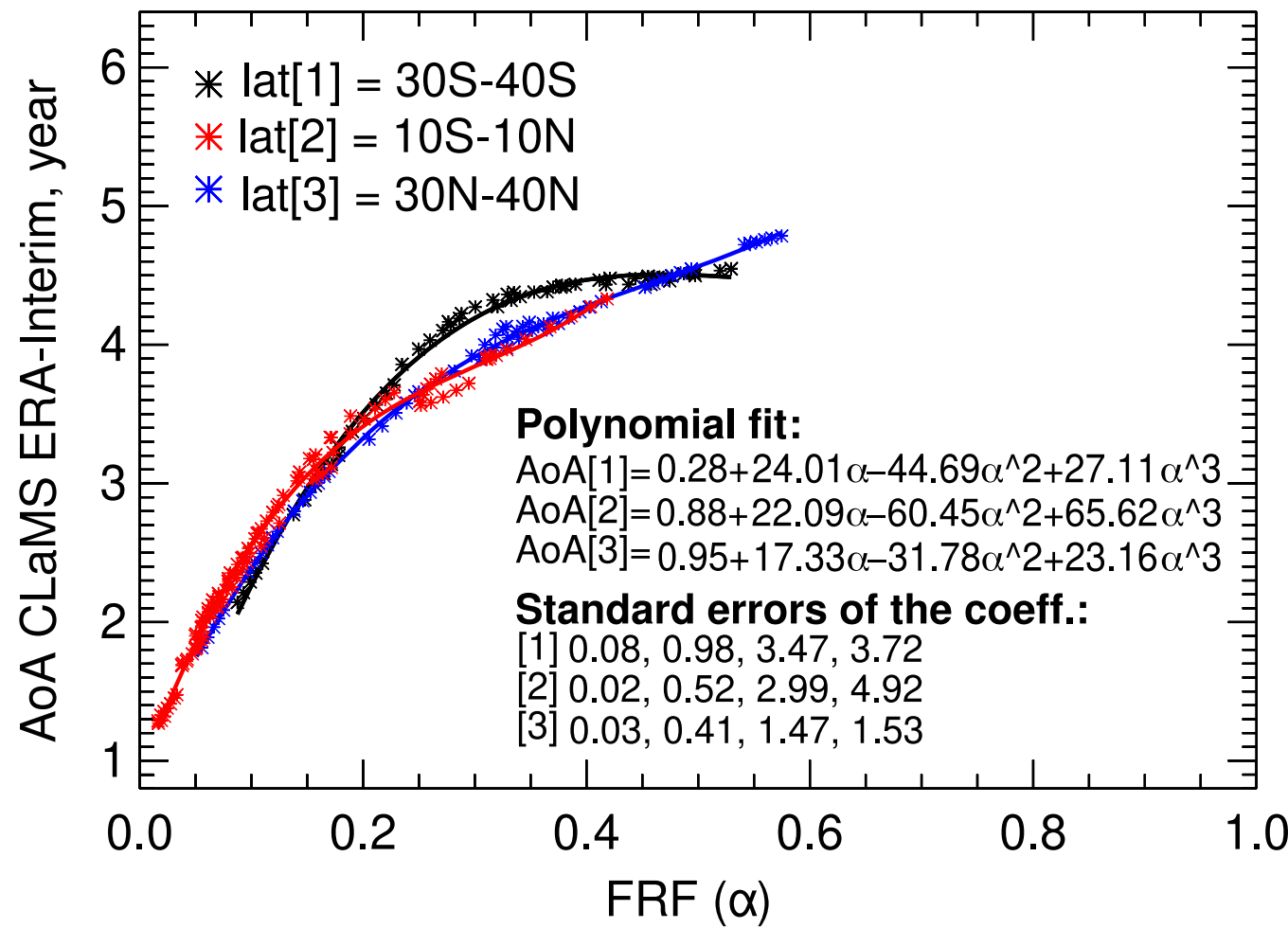
(b) AoA-FRF correlation (lat): JAN, 2000
