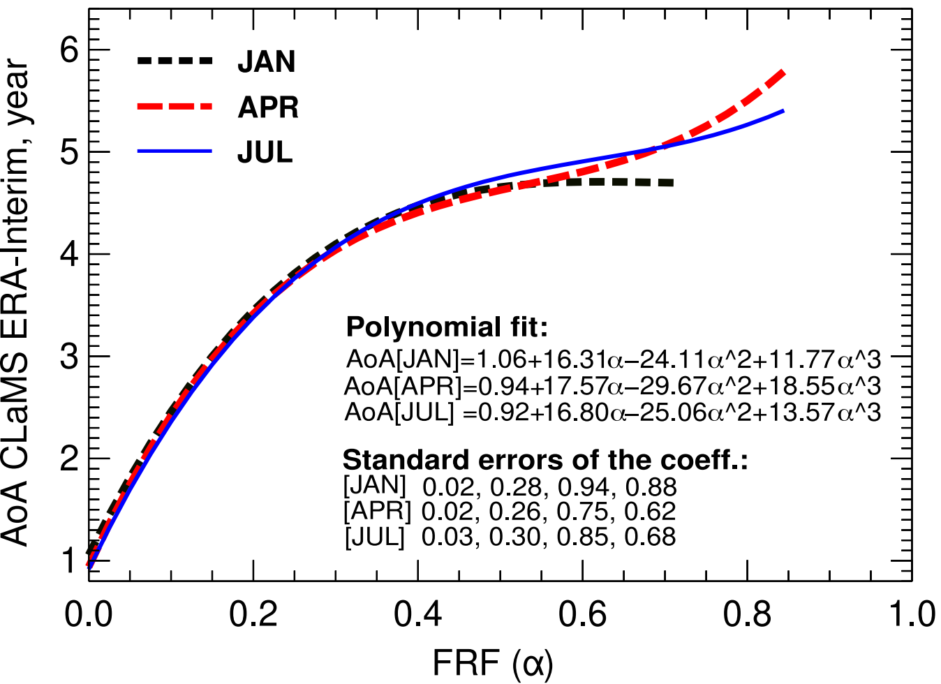
(a) AoA-FRF correlation by months: 1995
