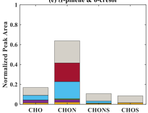
(e) \alpha -pinene & o-cresol
