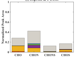
(f) Isoprene &amp; o-cresol
