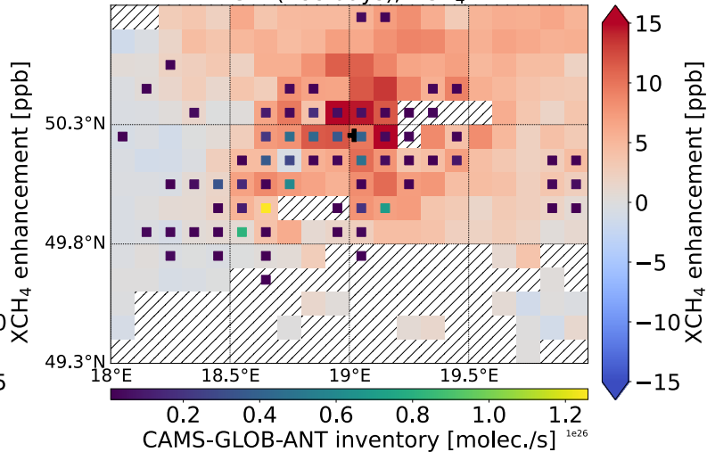
SW (288 days), XCH 4
