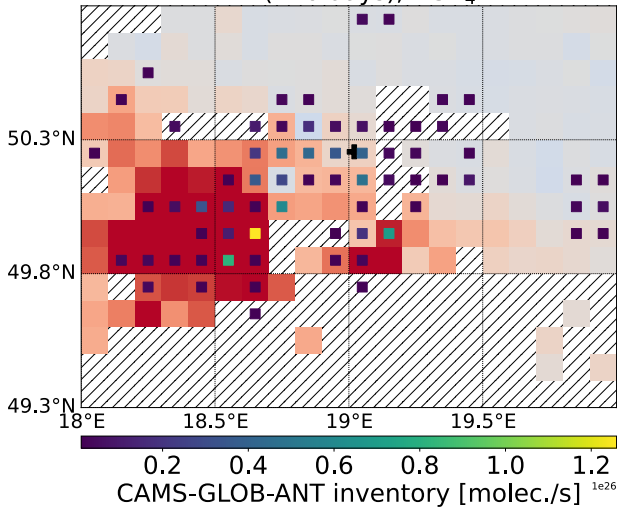
NE (226 days), XCH 4
