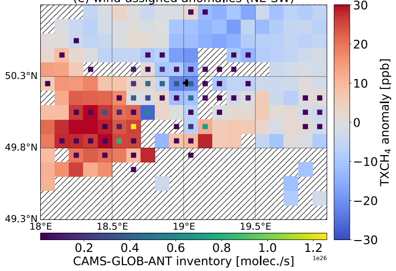
(e) wind-assigned anomalies (NE-SW)
