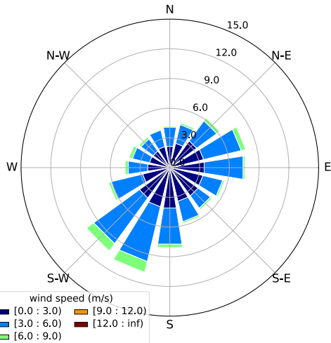
(a) ERA5 wind at 10 m
