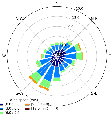
(b) ERA5 wind at 975 hPa (~330 m)
