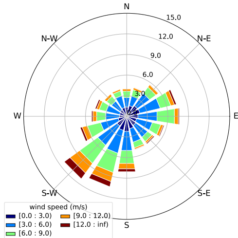
(c) ERA5 wind at 950 hPa (~500 m)
