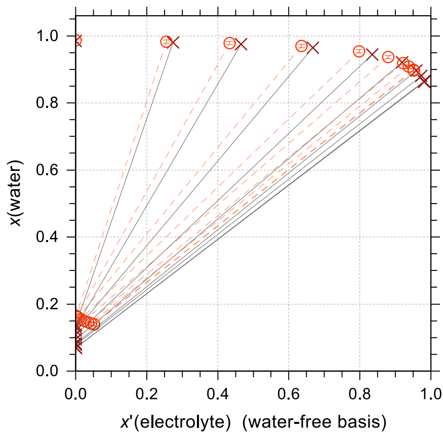
(b) H 2 O (1) + Ethyl acetate (2) + KI (3)
